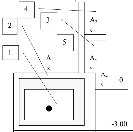
Fig. 1. Transverse section of accelerator building. 1 - tantalum converter, 2 - concrete shield, 3 - technological corridor, 4 - klystron hall, 5 - unattended room.
