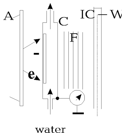
Fig.3. Scheme of measurement (scanned electron beam): A-accelerator LINAC-20; C-converter;
