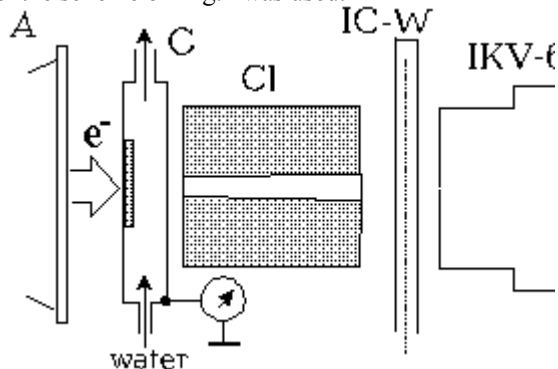
Fig.2. Scheme of measurement (not scanned electron beam): A-accelerator LINAC-10; C-converter; Cl- collimator (Pb, 200mm).
