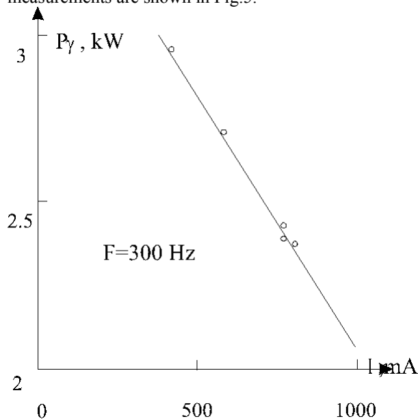
Fig. 4. Bremstrahlung power dependence on pulse current amplitude
