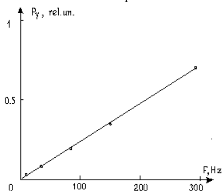
Fig. 5. Bremstrahlung power dependence of beam pulse repetition rate
