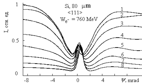
Fig. 3. The dependence of transmission and scattering of 760 MeV electrons through 80 \mu\text{m} Si single crystal on \langle 111 \rangle axis orientation. Registration solid angle is 1.2 \cdot 10^{-8} sr. The scattering angles \theta , radian: 1 – 0; 2 – 0.17 \cdot 10^{-3} ; 3 – 0.34 \cdot 10^{-3} ; 4 – 0.51 \cdot 10^{-3} ; 5 – 0.65 \cdot 10^{-3} ; 6 – 0.80 \cdot 10^{-3} ; 7 – 0.89 \cdot 10^{-3} ; 8 – 1.03 \cdot 10^{-3}
