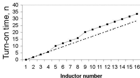
Fig. 5. Time diagram of LIA-10M inductors turn-on.
