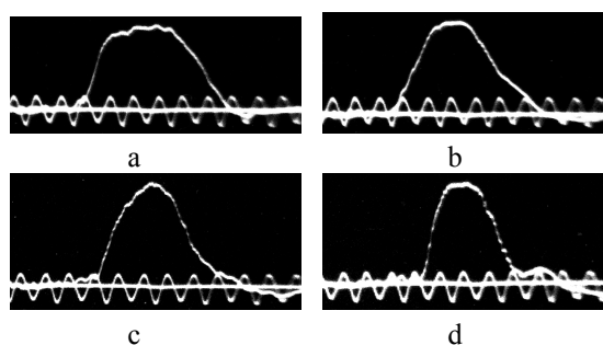
Fig. 2. Oscillograms of injected beam current pulses (duration at half-maximum: a – 40 ns, b – 35 ns, c – 30 ns, d – 25 ns).
