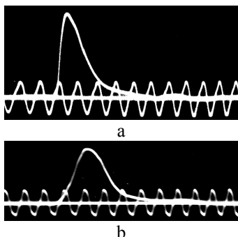
Fig. 3. Oscilloscope images of bremsstrahlung pulses corresponding to 25-ns (a) and 40-ns (b) duration of injection current pulses.
