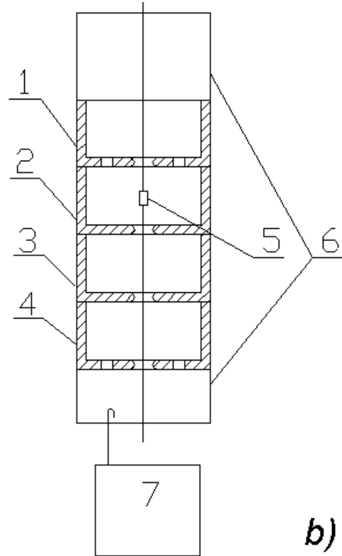
Fig. 1b. The measurement scheme of the coupling coefficient in the accelerating structure (1 – neighbor cell, 2, 3, 4 – cells of cascade tested, 5 – small metal detuning bead on the thread, 6 – absorbing cavities coated by al-sifer, 7 – analyzer).
