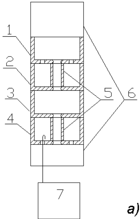
Fig. 1a. The scheme of frequency measurement of single cell (1, 2, 4 – neighbor cells, 3 – cell tested, 5 – shorting cylinders, 6 – absorbing cavities coated by al-sifer, 7 – analyzer).
