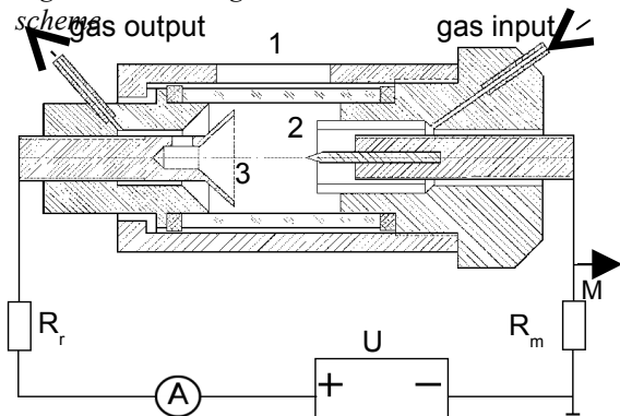
Fig.1. The discharge device sketch and the measuring
