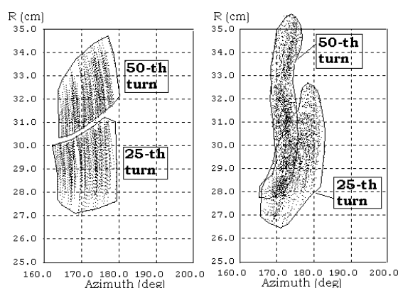
Fig. 5. Position of particles on the plane azimuth-radius during 25-th and 50-th turns. To the left – without taking into account space charge, to the right – taking into account it.
