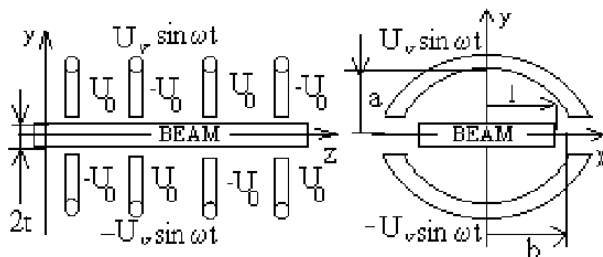
Fig. 1. The plane electrostatic undulator.
