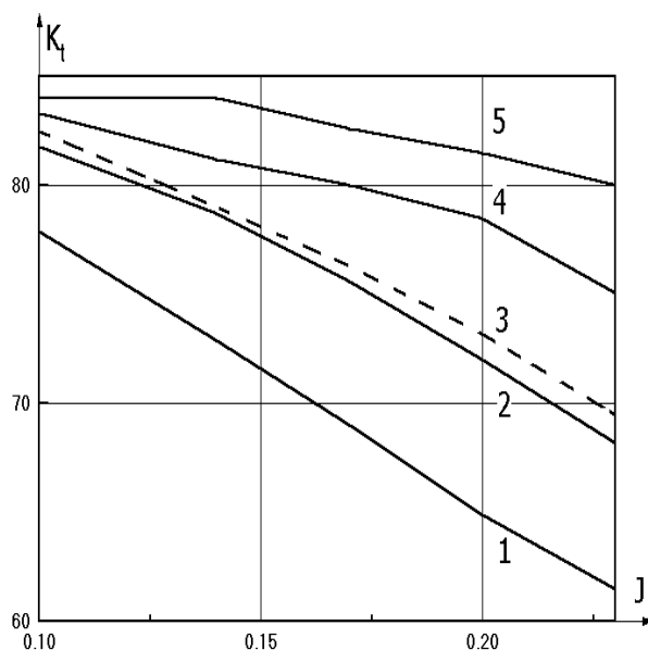
Fig. 5. Current transmission versus current density J \text{ (A/cm}^2\text{)} . Initial beam sizes: 1 - 2t \times 2l = 0.5 \times 12 \text{ cm}^2 , 2 - 2t \times 2l = 0.4 \times 12 \text{ cm}^2 , 3 - 2t \times 2l = 0.4 \times 14 \text{ cm}^2 , 4 - 2t \times 2l = 0.3 \times 12 \text{ cm}^2 , 5 - 2t \times 2l = 0.2 \times 12 \text{ cm}^2 .
