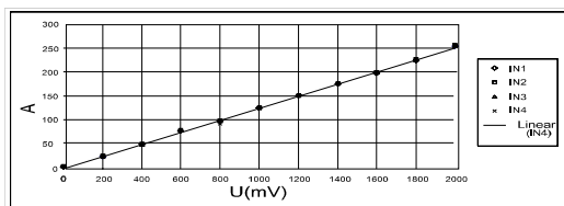
Fig. 4. Amplitude characteristics of four channels of one from the ADC modules
