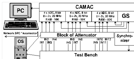
Fig. 3. Block diagram of the multichannel pulse-signal recording system
