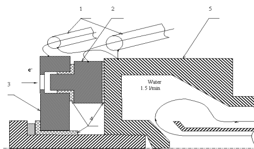
Fig. 2. The Faraday cup disposition diagram: 1 – coaxial lines, 2 – Faraday cup, 3 – mask, 4 – insulators, 5 – cooled chamber
