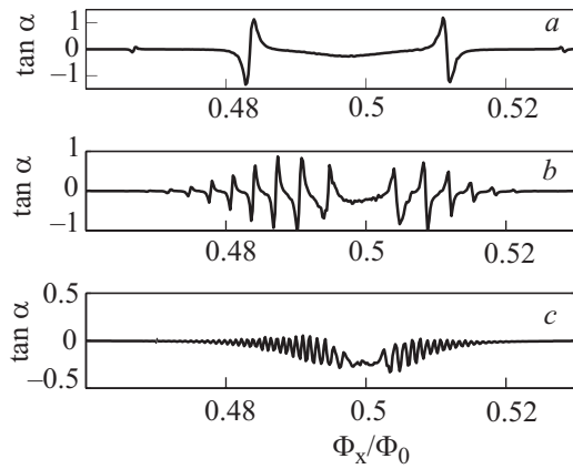
Fig. 3. The phase shift \alpha for the flux qubit excited by the series of rectangular pulses with: T = \tau = 0.5 (a), T = 0.5 , \tau = 5 (b), T = 0.5 , \tau = 20 (c).
