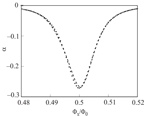
Fig. 4. Comparison of the theoretical (dashed) and numerical (marked by points) curves for the excitation with the series of the pulse with parameters: T = 0.5 , \tau = 100 .
