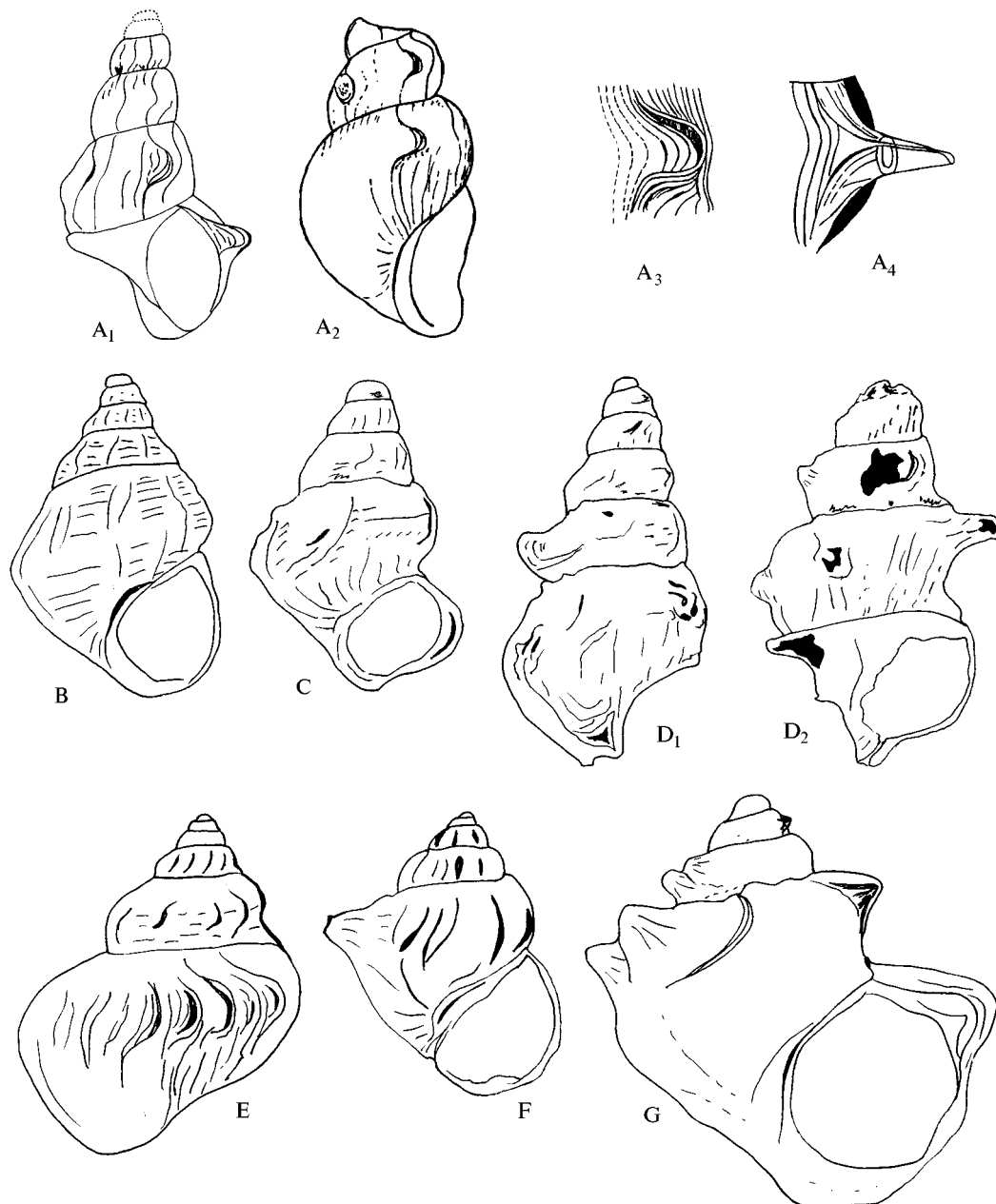
Fig. 3. The sculptural elements of Coelacanthia quadrispinosa (A 1 –A 4 ) and reconstructions of the morphological lineage Mohrensternia subinflata (B) — Coelacanthia quadrispinosa (C, D 1 , D 2 ) and Mohrensternia barboti (E) — Archaschenia merklini (F, G). B–D after Il'ina et al., 1976, modified; E–G after Zhgenti, 1991, modified.
