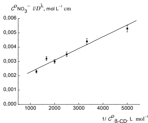
Fig. 4. Dependence of spectral characteristics of \text{NO}_3^- on amount of \beta\text{-CD} in aqueous solutions in coordinates of the Benesi-Hildebrand equation for inclusion compound of composition 1:1
