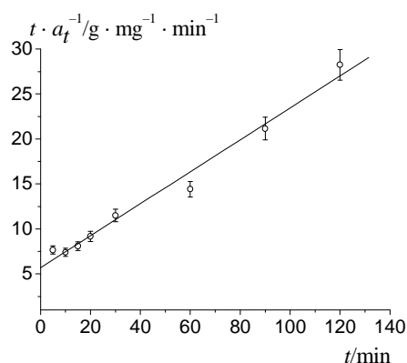
Fig. 6. Kinetic curve of Cd (II) cations sorption in the Lagergren pseudo-second order equation for adsorbent 3
