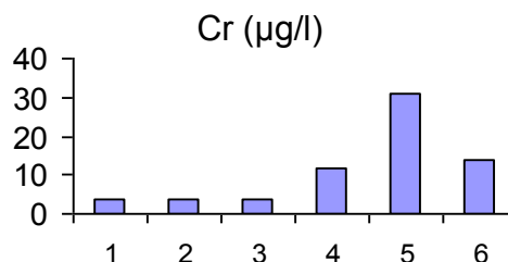
Fig. 1. Graphs of changes in chromium content in water from the loop in the period 17-22.08.2019
