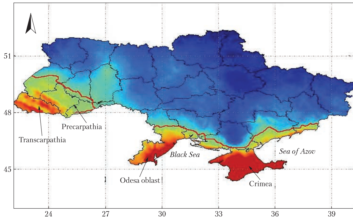
Ensemble map for the predicted distribution of the Asian tiger mosquito, Aedes albopictus , in Ukraine. Red color indicates areas of higher bioclimatic suitability, whereas blue indicates the opposite; the red line represents the accepted threshold
