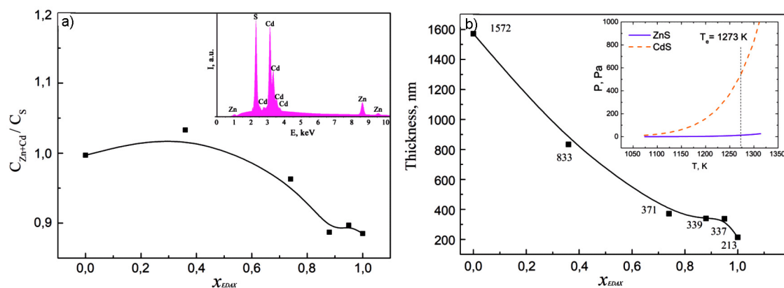
Fig. 5. The dependence of the films stoichiometry C_{\text{Zn+Cd}}/C_S on zinc content x_{EDX} , which was indicated by EDX method (a) and thickness of \text{Zn}_x\text{Cd}_{1-x}\text{S} films with different zinc concentrations x_{EDX} (b). The typical characteristic EDX spectra of \text{Zn}_x\text{Cd}_{1-x}\text{S} solid solutions films and dependences of ZnS and CdS gas pressure on temperature are presented on insets.
