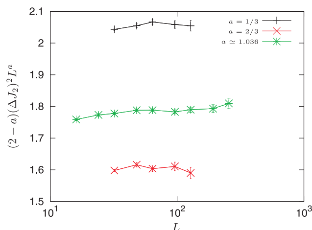
Figure 4. (Color online) Amplitude w of disorder correlations (up to a factor (J_1 - J_2)^2/4 ) versus the lattice size L . Different curves correspond to different disorder correlations, i.e., to different exponents a = 1/3 , 2/3 and 1.036 .
