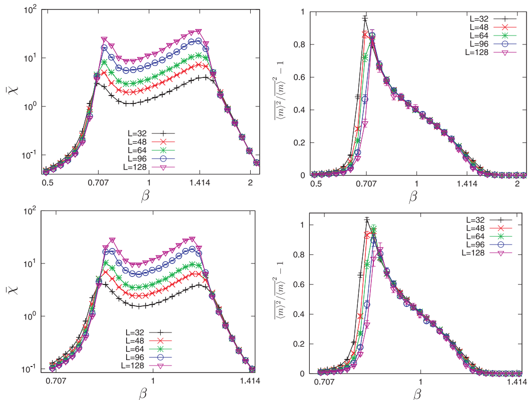
Figure 5. (Color online) On the left, average magnetic susceptibility of the 8-state Potts model with a disorder correlation exponent a = 2/3 and a disorder strengths r = J_1/J_2 = 3.5 (top) and r = 2 (bottom). Different curves correspond to different lattice sizes. On the right, ratio R_m = \overline{\langle m \rangle^2} / \langle m \rangle^2 - 1 for the same models. Note that the horizontal scales are not the same.
