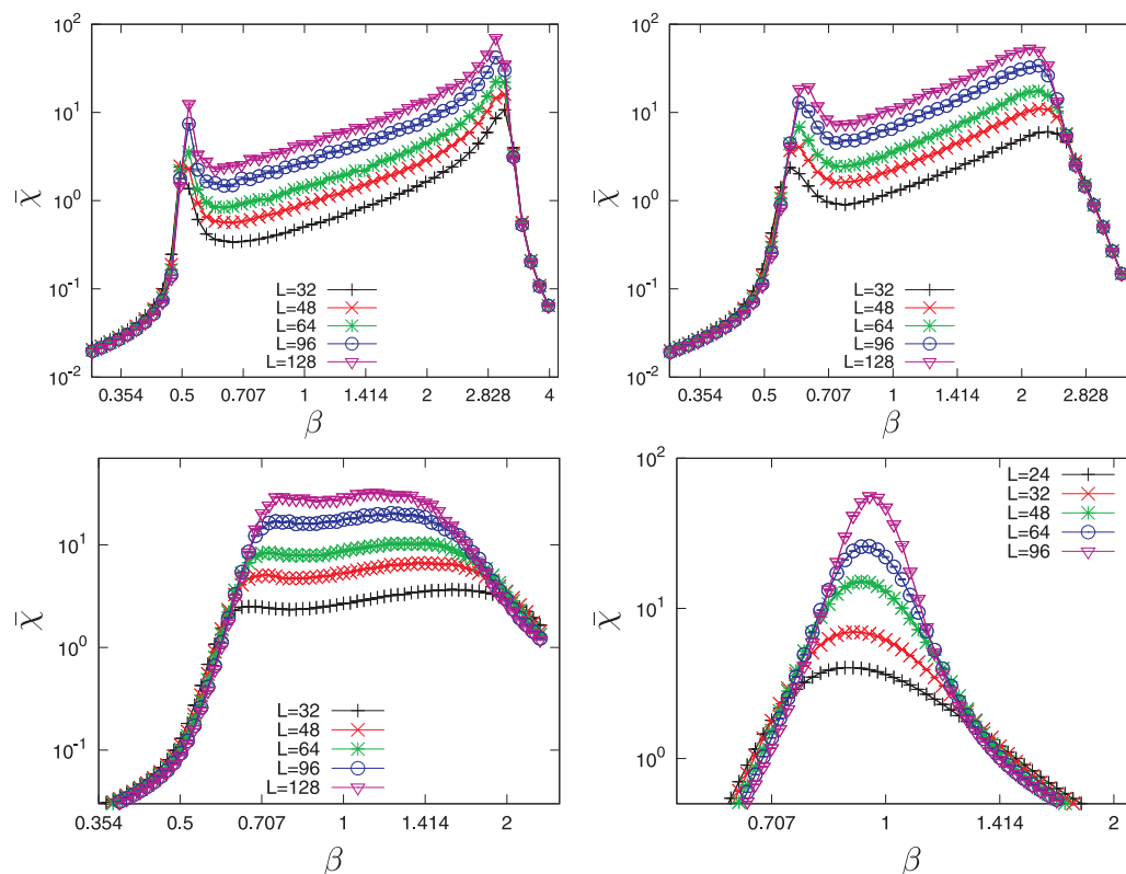
Figure 1. (Color online) Average magnetic susceptibility of the 8-state Potts model with different disorder correlation exponents ( a = 1/3, 2/3, 1.036 and 2 from left to right and top to bottom) for a disorder strength r = J_1/J_2 = 7.5 . The different curves correspond to different lattice sizes. Note that the scale of the y-axis is logarithmic.
