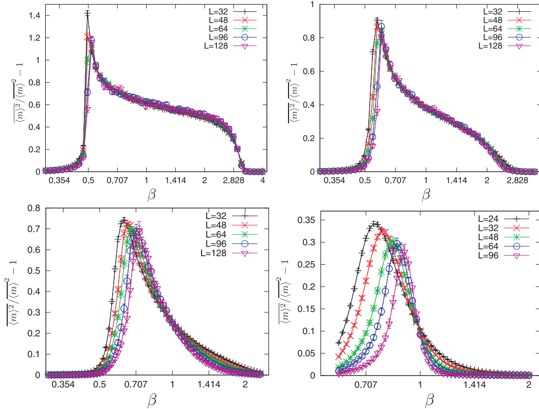
Figure 3. (Color online) Ratio \overline{\langle m \rangle^2} / \langle \overline{m} \rangle^2 - 1 of the 8-state Potts model with different disorder correlation exponents ( a = 1/3, 2/3, 1.036 and 2 from left to right and top to bottom) for a disorder strength r = J_1/J_2 = 7.5 . Different curves correspond to different lattice sizes.
