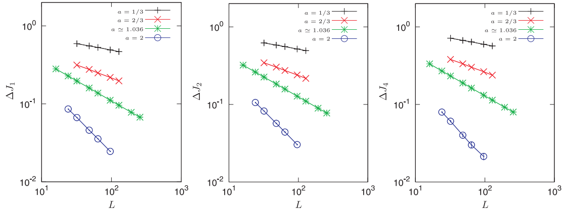
Figure 2. (Color online) Fluctuations \Delta J (up to a factor (J_1 - J_2)/2 ) of the average random couplings versus the lattice size L . Different curves correspond to different disorder correlations, i.e., to different exponents a = 1/3, 2/3, 1.036 and 2 (from top to bottom).
