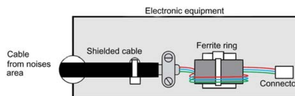
Fig. 4. Ferrite Ring Filter Installed on a Control Cable Entering the Electronic Equipment
