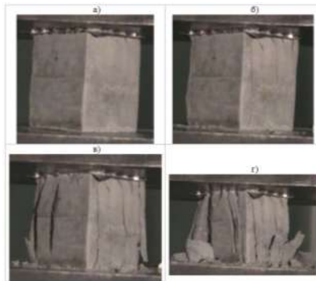
а – \sigma_{\bar{n}e} = 17 \bar{H}\bar{a} , \Delta h = 1 \div 2\% ; б – \sigma_{\bar{n}e} = 22 \bar{H}\bar{a} (максимальная), \Delta h = 3\% ; в – \sigma_{\bar{n}e} = 8 \bar{H}\bar{a} , \Delta h = 10\% ; г – \sigma_{\bar{n}e} = 5 \div 6 \bar{H}\bar{a} , \Delta h = 20 \div 30\%
