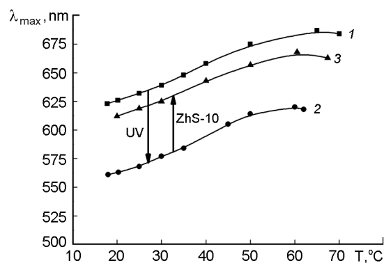
Fig. 2. Selective reflection maximum \lambda_{max} as function of temperature for 25 % M5 + 75 % ZhK-440 before (1) and after (2,3) irradiation. 2 — UV irradiation without filter, 10 mW/cm 2 ; 3 — light irradiation using filter ZhS-10, 10 mW/cm 2 .
