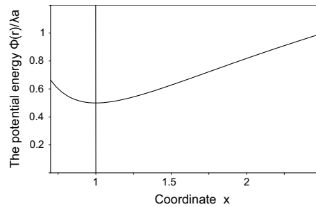
Figure 3. The dependence of the potential energy on the dimensionless coordinate x = r/r_0 . Here \beta = 10^{-2} and \gamma = 5 \cdot 10^{-5} .
