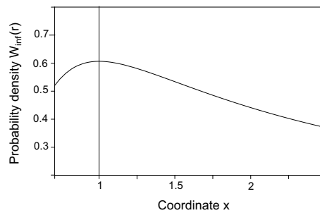
Figure 4. The dependence of the probability density on the dimensionless coordinate x = r/r_0 . Here \beta = 10^{-2} and \gamma = 5 \cdot 10^{-5} .
