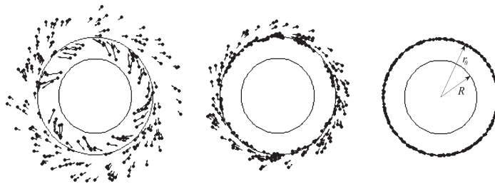
Figure 1. The distribution of non-interacting spherical particles ( N=200 ) in the hydrodynamic field of a swirling flow at different times. The circle of radius r_0 represents the equilibrium orbit.
