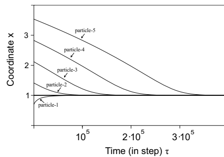
Figure 2. The dependence of the dimensionless radial coordinate x = r/r_0 on the number of time steps \tau = t\lambda ( N=5 ), \beta = \omega/\lambda = 10^{-2} , \gamma = V/(\lambda R) = 5 \cdot 10^{-5} .
