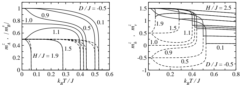
Figure 5. Temperature dependences of the reduced components m_B^s , m_A^z of the order-parameter and the reduced sublattice magnetization m_{Bh}^z , m_{Bv}^z for the decorated superexchange antiferromagnetic model with S = 3/2 , D/J = -0.5 and some typical values of the magnetic field.
