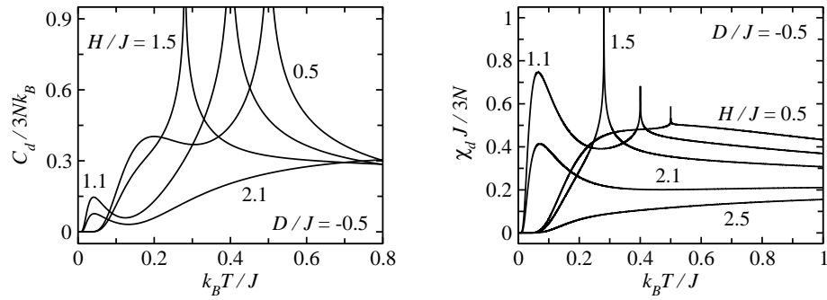
Figure 6. Temperature dependences of the reduced specific heat and susceptibility for the decorated superexchange antiferromagnetic model with S = 3/2 , D/J = -0.5 and some typical values of the magnetic field.
