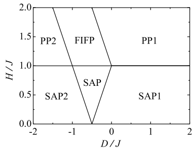
Figure 2. Ground-state phase diagram in the D-H plane for the decorated superexchange antiferromagnetic model with S = 3/2 .
