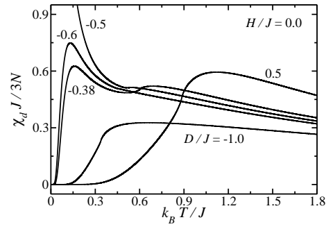
Figure 4. Temperature dependences of the reduced initial susceptibility for the decorated superexchange antiferromagnetic model with S = 3/2 and some typical values of the crystal field.
