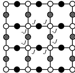
Figure 1. Part of the decorated square lattice with vertex spin 1/2 (open circles) and decorating spins 3/2 (closed and obliquely lined circles). J denotes the exchange interaction which is antiferromagnetic (ferromagnetic) in the horizontal (vertical) direction.
