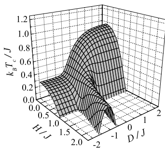
Figure 3. Global phase diagram in the D-H-T space for the decorated superexchange antiferromagnetic model with S = 3/2 .
