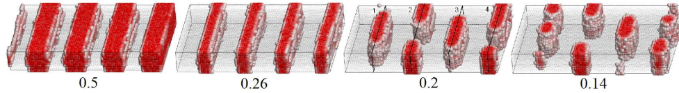
Figure 4. (Color online) Sequence of morphologies obtained for d = 13.333 and w = 10 at various fractions f_B (indicated at the bottom). Blocks of B beads filling the space between pillars of A beads ( f_B = 0.50 ), thinned blocks ( f_B = 0.26 ), hexagonally arranged columns ( f_B = 0.20 ), and random columns ( f_B = 0.14 ) are shown. Only color-coded density of B beads is displayed.
