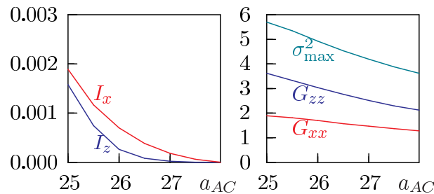
Figure 7. (Color online) Behavior of the overlap integrals I_x and I_z (left hand frame) and the components G_{xx} and G_{zz} and maximal eigenvalue \sigma_{\max}^2 of the gyration tensor (right hand frame) upon the changes of the quality of the one-component solvent. The quality of the solvent is defined via the repulsion parameter a_{AC} between polymer (A) and solvent (C) beads, the value of a_{AC} = 25 represents the case of a good solvent.
