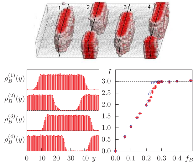
Figure 5. (Color online) Left bottom frame shows the density profiles \rho_B^{(i)}(y) along each i -th slab region shown in the top frame. Right bottom frame shows the dependence of the integral profile I (averaged over four slabs) on f_B . The results for simulation set I are shown as blue disks and for the set II — as red asterisks.
