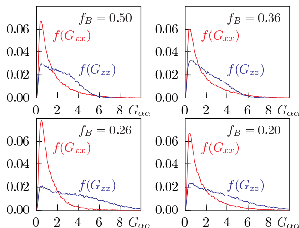
Figure 12. (Color online) Distributions of the relevant gyration tensor components, G_{xx} and G_{zz} for various fractions f_B (indicated in each frame). The case of d = 20 , w = 13 and out-of-phase arrangement of stripes is shown.
