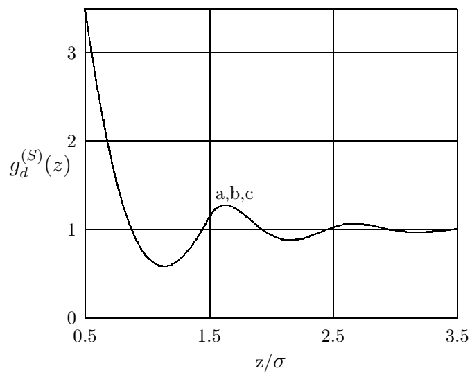
Figure 3. The S-part of solvent density profiles at c_1 = 0.0115 .
