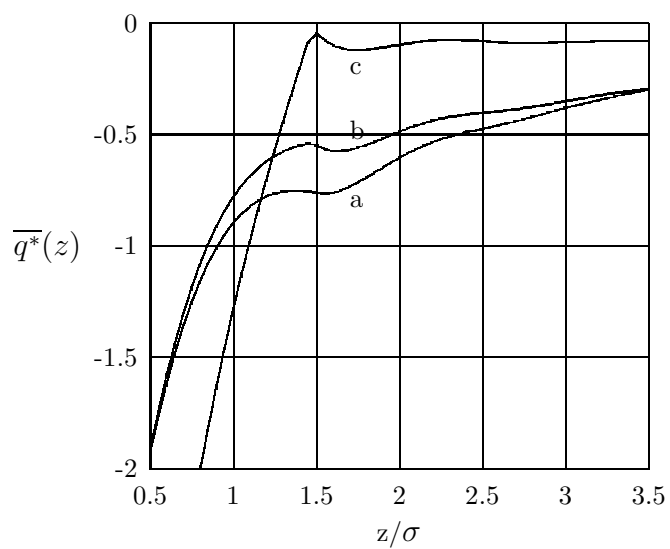
Figure 4. The charge profiles at c_1 = 0.0115 .
