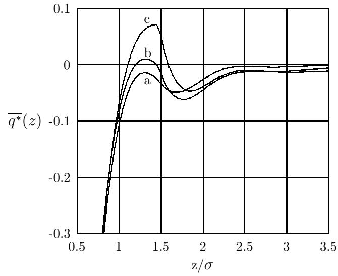
Figure 5. The charge profiles at c_1 = 0.11 .
