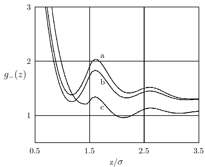
Figure 2. The density profiles of anions at c_1 = 0.0115 .
