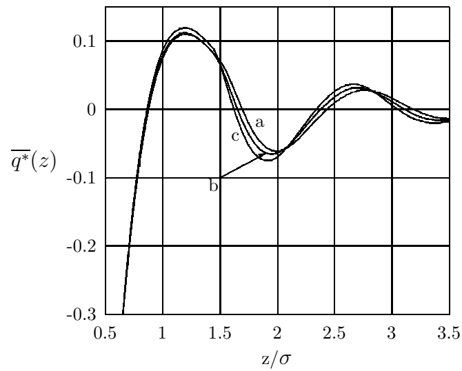
Figure 6. The charge profiles at c_1 = 0.5 .
