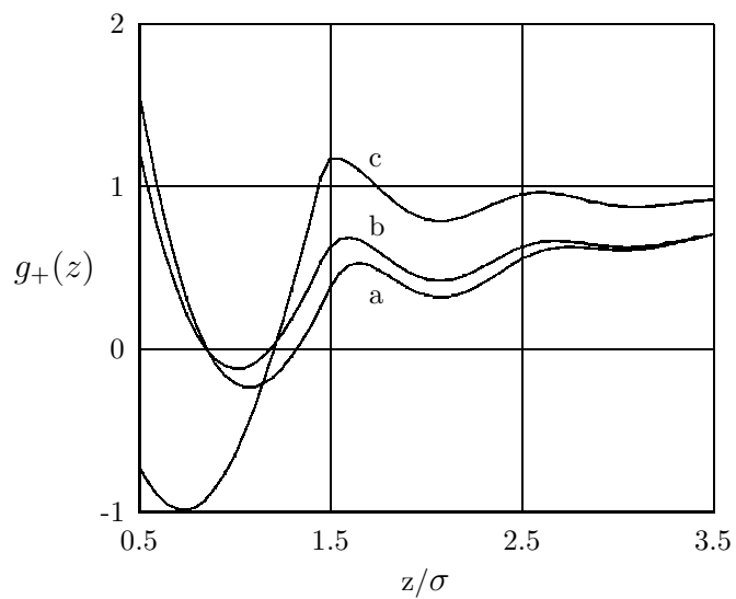
Figure 1. The density profiles of cations at c_1 = 0.0115 .
