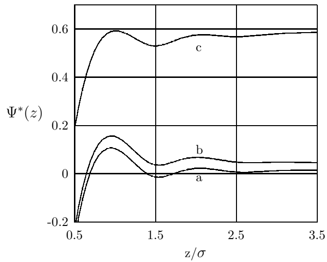
Figure 8. The potential profiles at c_i = 0.0115 .
