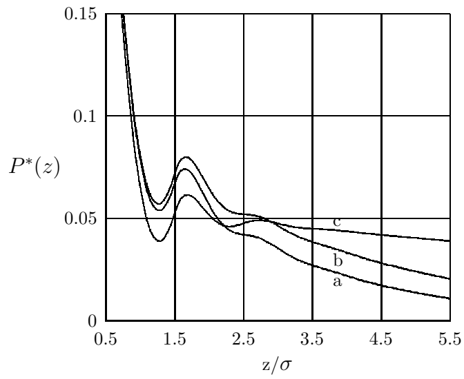
Figure 7. The polarization profiles at c_i = 0.0115 .
