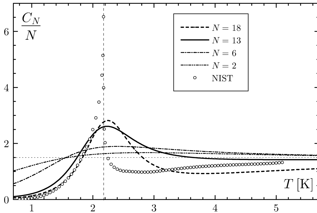
Figure 3. Heat capacities in the free volume and circular approximation. The circles show the NIST C_V data [18].
