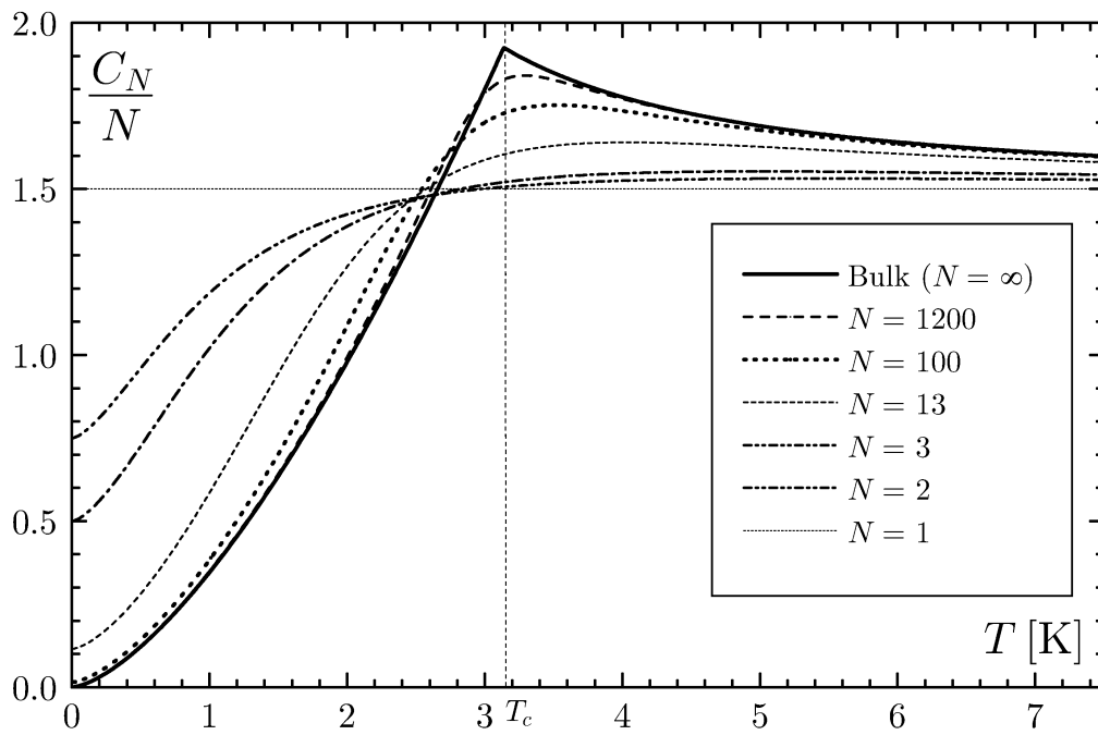
Figure 1. Heat capacities in the ideal case.
