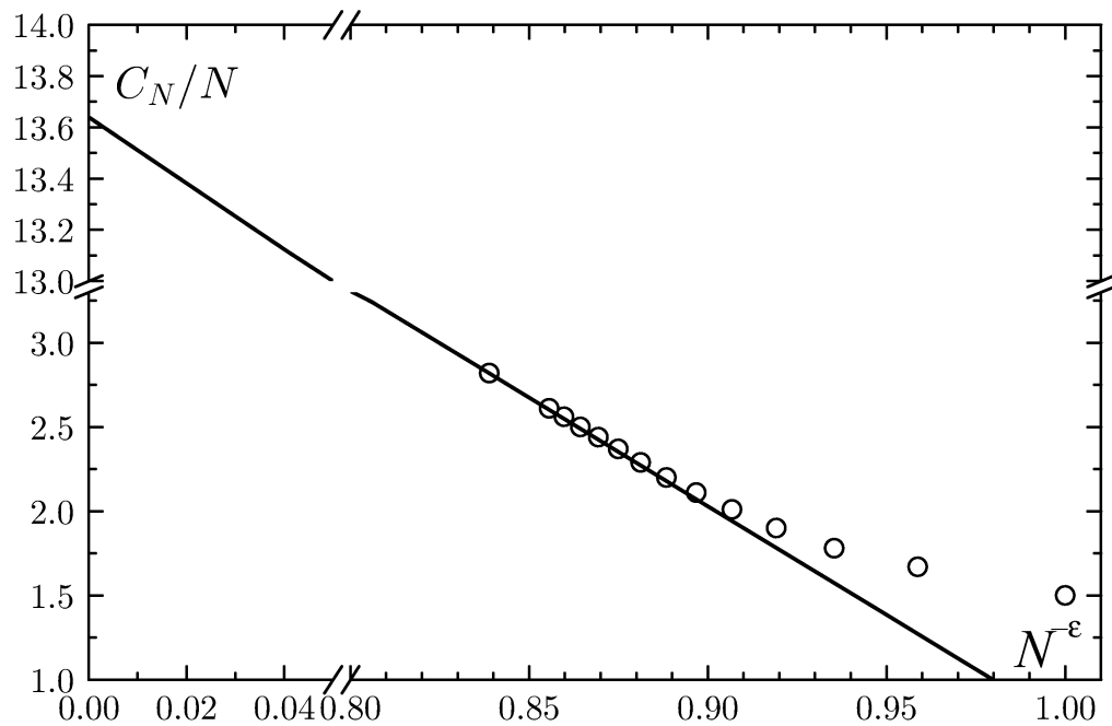
Figure 4. C_N^{\max}/N values for the hard spheres system. Solid line shows dependence (29), circles correspond to the data from table 2.
