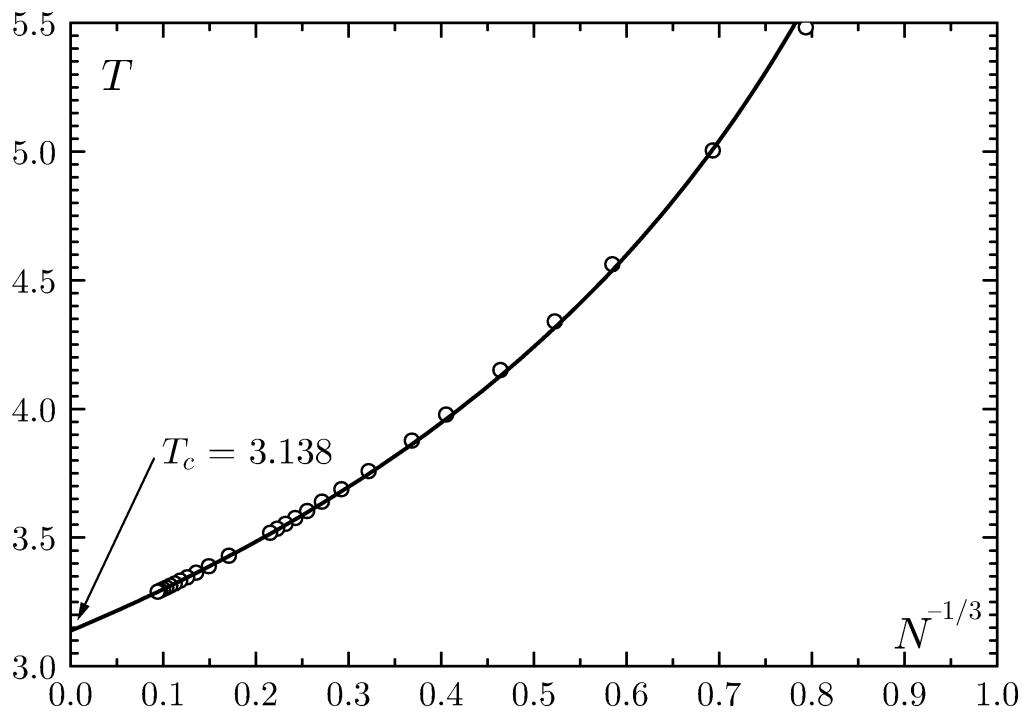
Figure 2. Temperature of the C_N/N maxima in the ideal case. Solid line shows dependence (20), circles correspond to the data from table 1.
