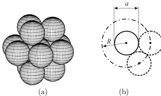
Figure 5. Helium-4 atoms as hard spheres. (a) The first closed sphere of 12 atoms surrounding 1 central atom. One atom is not seen since it is situated exactly behind the central atom. (b) Solid line shows the “surface of atom”, dashed line shows the “surface of alien atoms”, dashed-dotted line shows “surface of inaccessible space”. Thus, assuming the volume of “inaccessible space” 4\pi R^3/3 to be the volume occupied by 1 atom one can obtain the hard sphere diameter a \simeq 2.2 \text{ \AA} .
