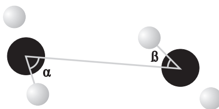
Figure 5. The uranyl-uranyl mutual orientation and characteristic angles.
