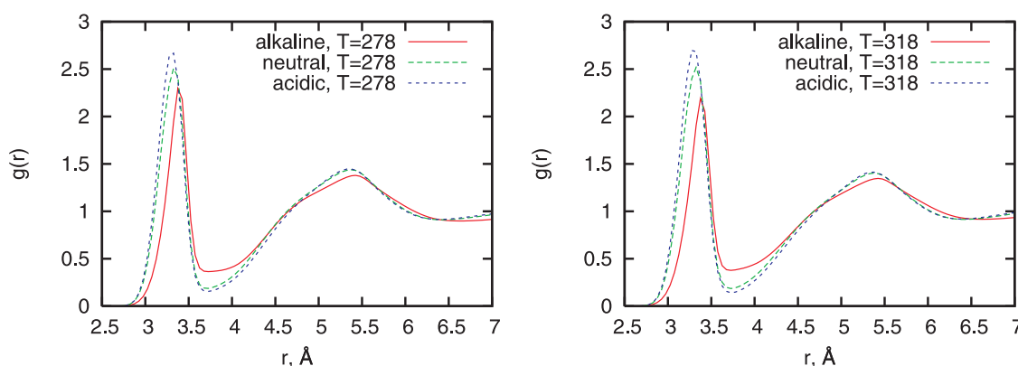
Figure 2. (Color online) The uranium-hydrogen (of water, \text{OH}^- and \text{H}^+ ions) RDFs for T = 278 K (left) and 318 K (right). The color scheme is the same as in figure 1.
