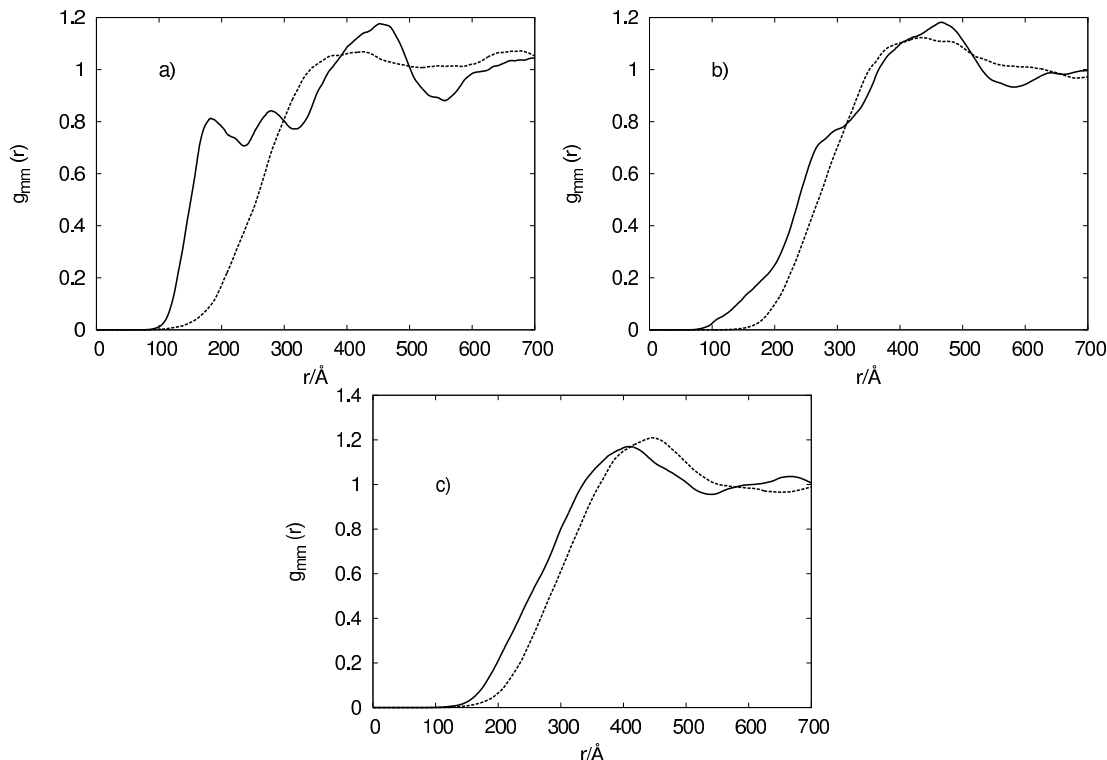
Figure 6. Intermolecular monomer-monomer pair distribution function for N_m = 48 at r_c = 1 \text{\AA} (a), 2 \text{\AA} (b), and 3 \text{\AA} (c) for flexible (continuous line) and rigid chains (dashed line).
