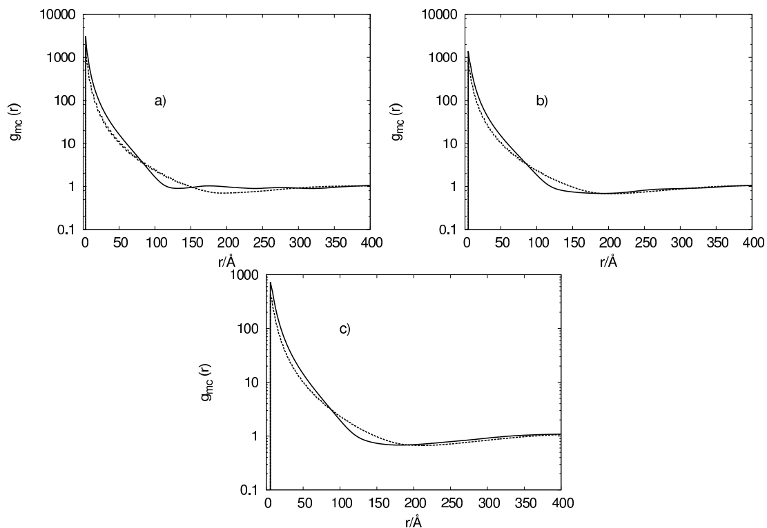
Figure 7. Monomer-counterion pair distribution function for N_m = 48 at r_c = 1 \text{ \AA} (a), 2 \text{ \AA} (b), and 3 \text{ \AA} (c) for flexible (continuous line) and rigid chains (dashed line).
