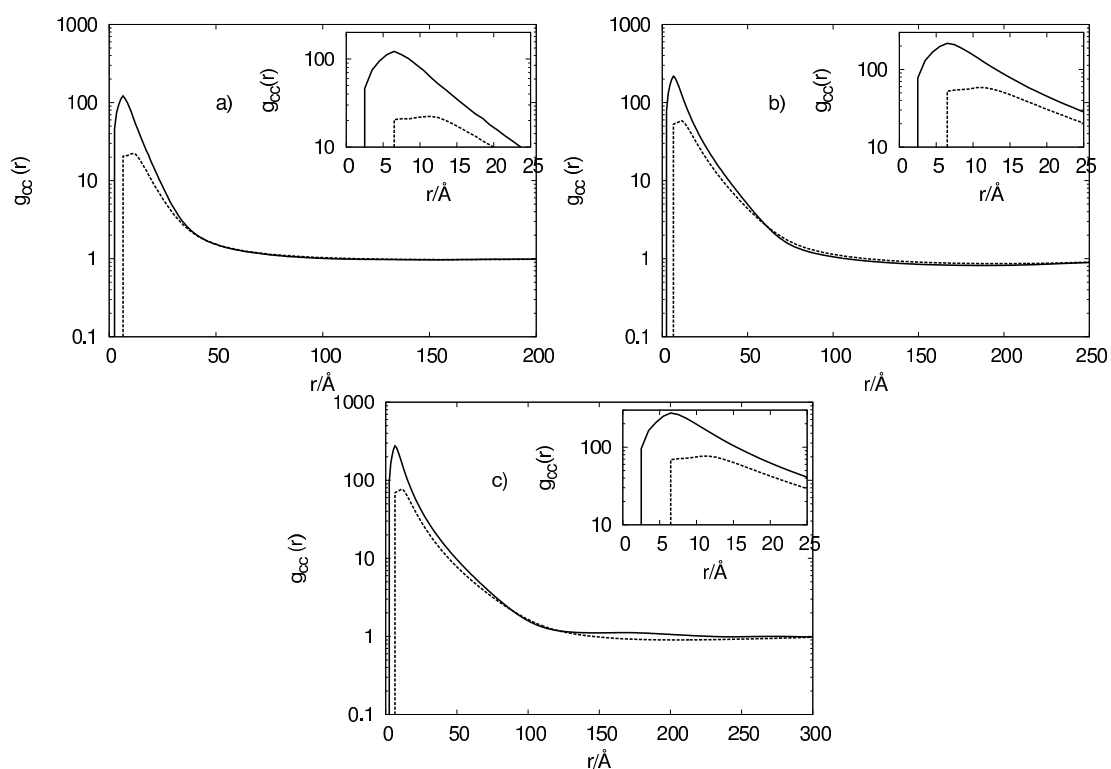
Figure 5. Counterion-counterion pair distribution function at N_m = 16 (a), 32 (b), and 48 (c) all for r_c = 1 \text{ Å} (continuous line) and 3 \text{ Å} (dashed line).
