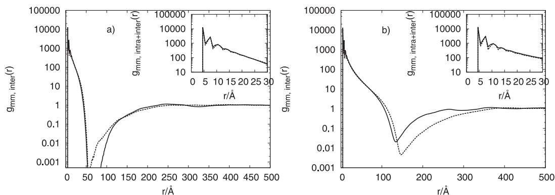
Figure 3. Intermolecular monomer-monomer pair distribution function for N_m = 16 (a) and N_m = 48 (b), for r_c = 1 \text{ \AA} (continuous line) and 3 \text{ \AA} (dashed line). Insets show the total (intermolecular plus intramolecular) distribution at short separations.
