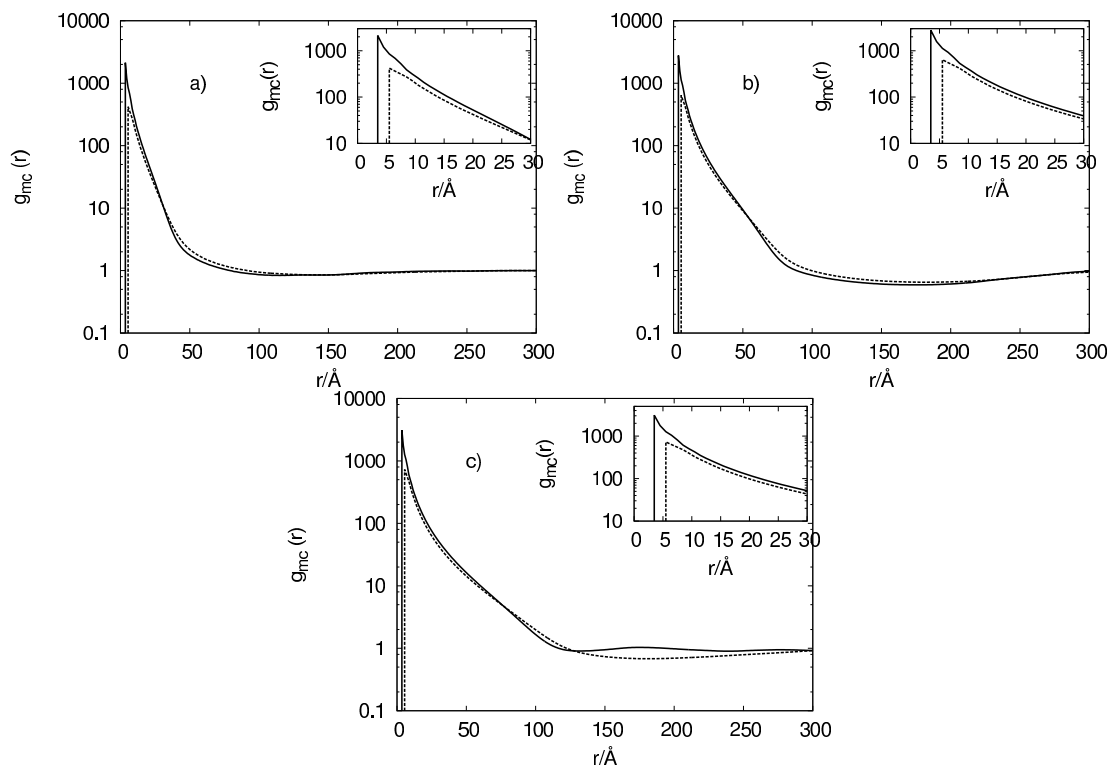
Figure 4. Monomer-counterion pair distribution function at N_m = 16 (a), 32 (b), and 48 (c), all for r_c = 1 \text{ Å} (continuous line) and 3 \text{ Å} (dashed line).
