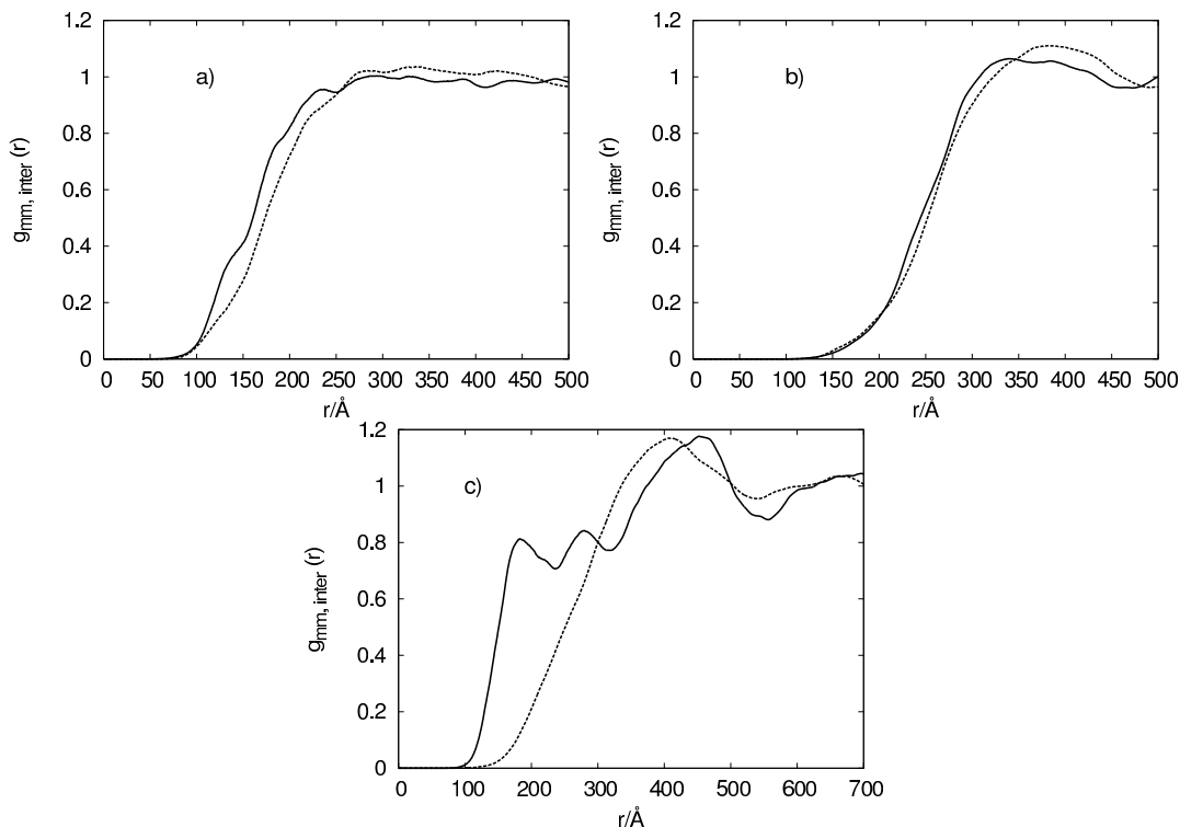
Figure 2. Intermolecular monomer-monomer pair distribution function at N = 16 (a), 32 (b), and 48 (c), for r_c = 1 \text{ \AA} (continuous curve) and 3 \text{ \AA} (dashed curve).
