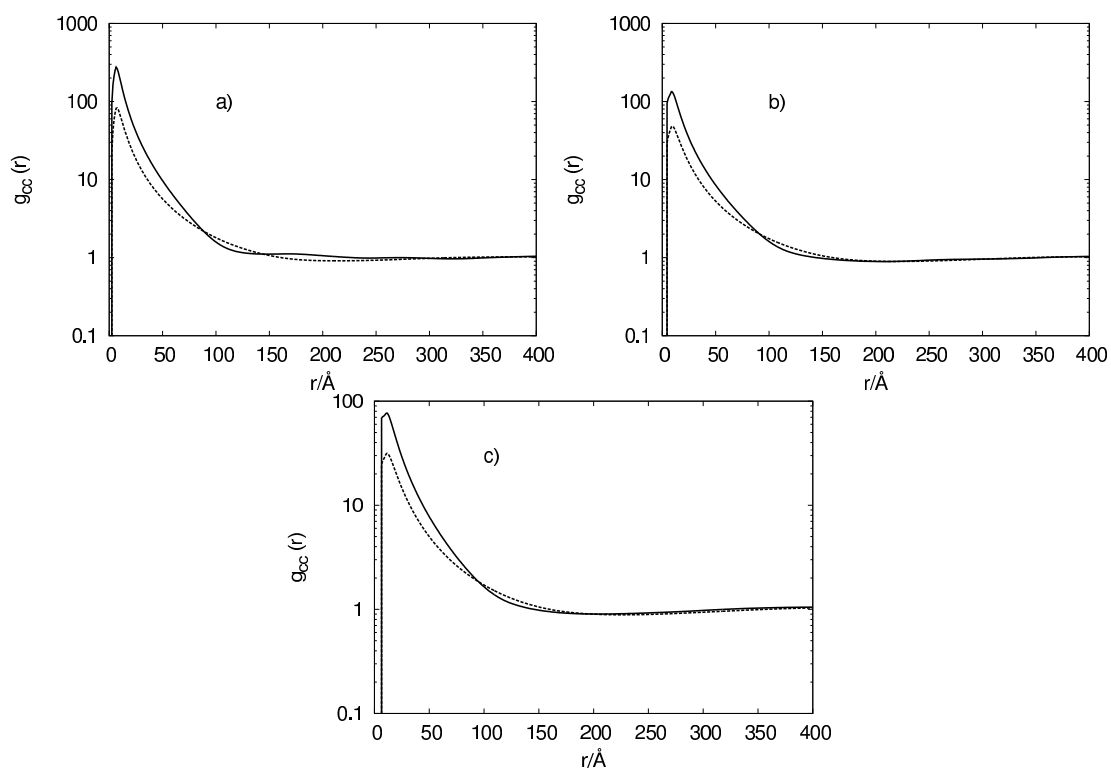
Figure 8. Counterion-counterion pdf for N_m = 48 at r_c = 1 \text{ \AA} (a), 2 \text{ \AA} (b), and 3 \text{ \AA} (c) for flexible (continuous line) and rigid chains (dashed line).
