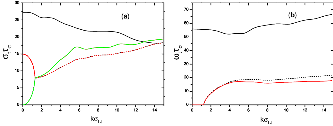
Figure 1. Generalized transverse mode spectrum of the LJ fluid at n^* = 0.845 and T^* = 1.705 : (a) damping coefficients and (b) dispersions. The results of two- and four-mode approximations are plotted by dashed and solid lines, respectively. From [24].
