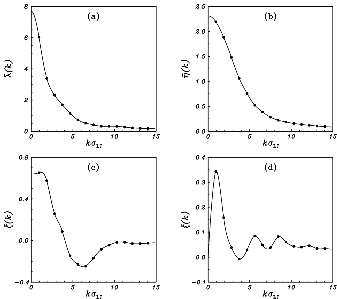
Figure 4. Reduced k -dependent transport coefficients of the LJ fluid at n^* = n\sigma_{LJ}^3 = 0.845 and T^* = k_B T / \epsilon_{LJ} = 1.706 , namely, the generalized thermal conductivity (a), the generalized shear (b) and the bulk (c) viscosities, and the cross correlation coefficient (d). From [27].
