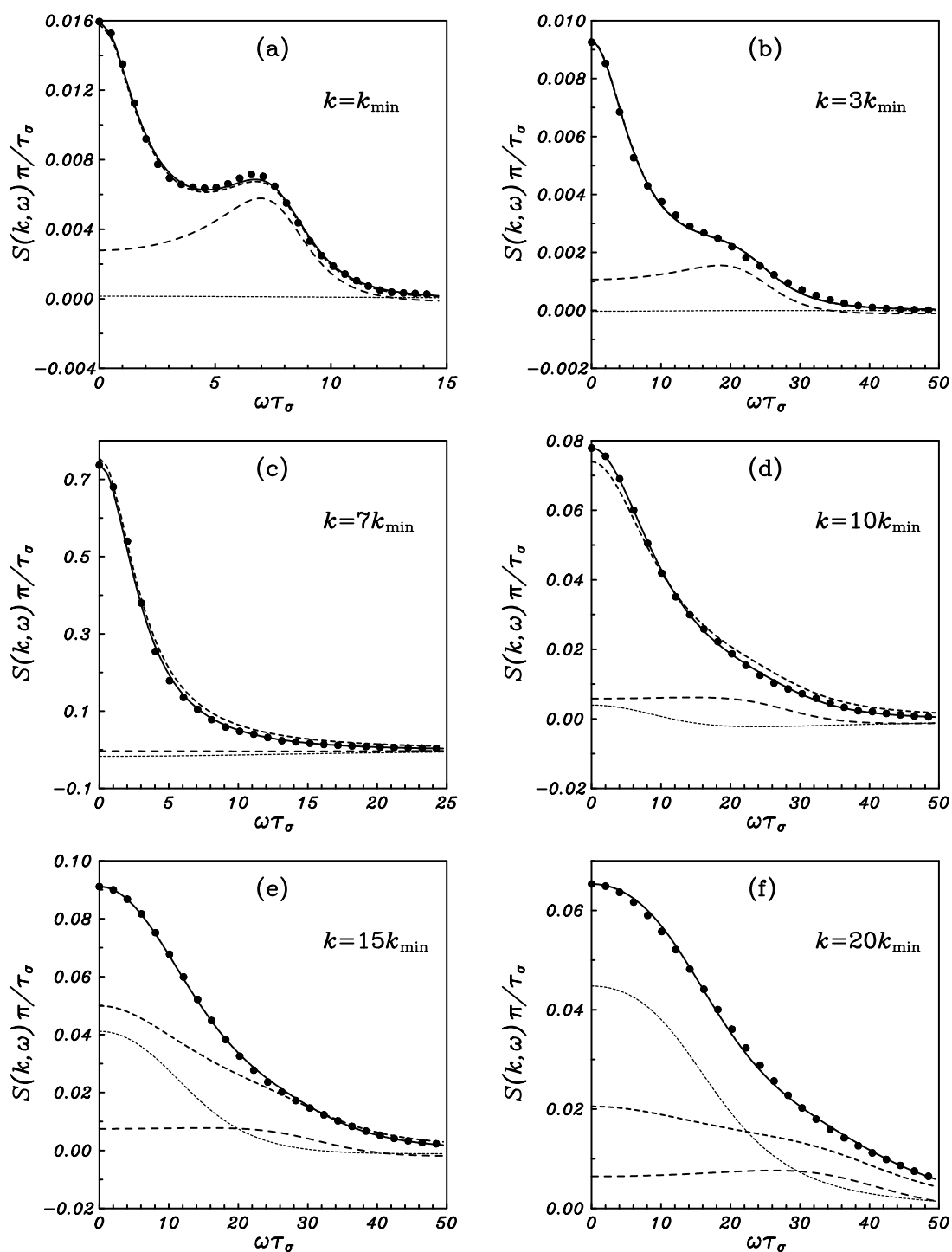
Figure 3. Dynamic structure factor of the LJ fluid at n^* = n\sigma_{LJ}^3 = 0.845 and T^* = k_B T / \epsilon_{LJ} = 1.706 as a function of \omega\tau_\sigma for six values of k\sigma_{LJ} : (a) k\sigma_{LJ} = 0.936 , (b) k\sigma_{LJ} = 2.807 , (c) k\sigma_{LJ} = 6.549 , (d) k\sigma_{LJ} = 9.355 , (e) k\sigma_{LJ} = 14.033 , (f) k\sigma_{LJ} = 18.710 . The results of the nine-mode approximation are plotted by the solid curve. The separated contributions from the kinetic, generalized hydrodynamic and generalized sound modes are indicated by the dotted, dashed, and long-dashed curves, respectively. From [26].
