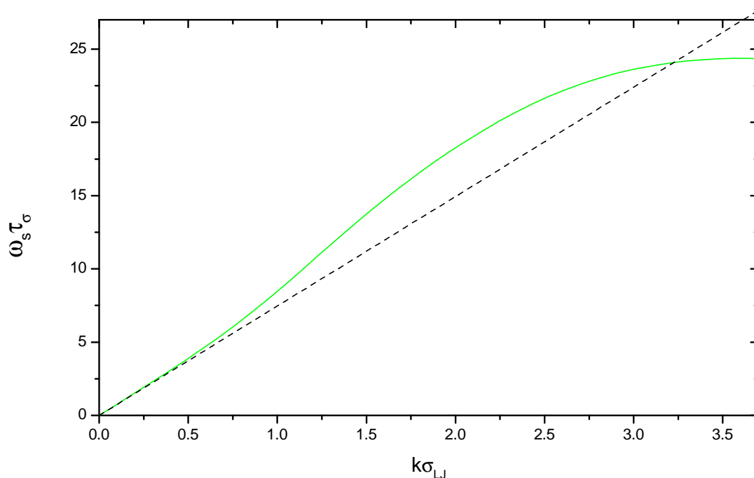
Figure 5. Sound dispersion of the LJ fluid at n^* = 0.845 and T^* = 1.705 . The results of the nine-mode description are shown by the solid curve and the hydrodynamic dispersion \omega_s^{\text{hyd}} = c_s k is plotted by the dashed line.
