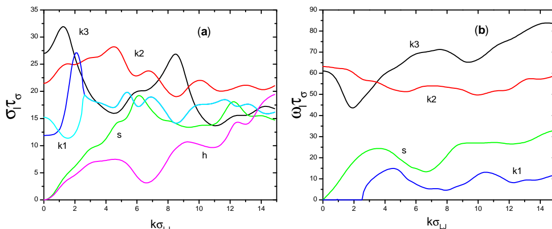
Figure 2. Generalized longitudinal mode spectrum of a LJ fluid in the nine-mode description at n^* = 0.845 and T^* = 1.705 : (a) damping coefficients and (b) dispersions. Note that two kinetic (k1) modes start as two purely relaxing modes and become complex-conjugated ones for k\sigma_{LJ} > 2.5 . From [24].
