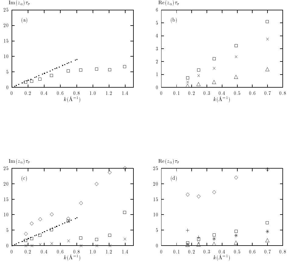
Figure 6. Generalized collective mode spectra obtained for hydrodynamic (a,b) and extended (c,d) sets of dynamic variables for a \text{He}_{0.65}\text{Ne}_{0.35} mixture. The linear dispersion of sound with c_s = 362 m/s is plotted by a dotted line. The imaginary (a, c) and real (b, d) parts of the eigenvalues are shown for: sound modes by boxes; concentration modes by triangles; ‘fast sound’ modes by diamonds; ‘slow sound’ modes by \times . From [30].
