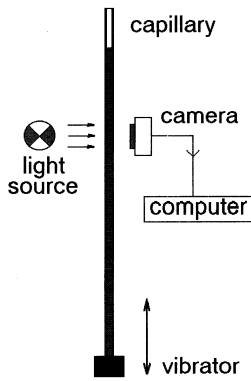
Figure 1. The schematic experimental setup.
