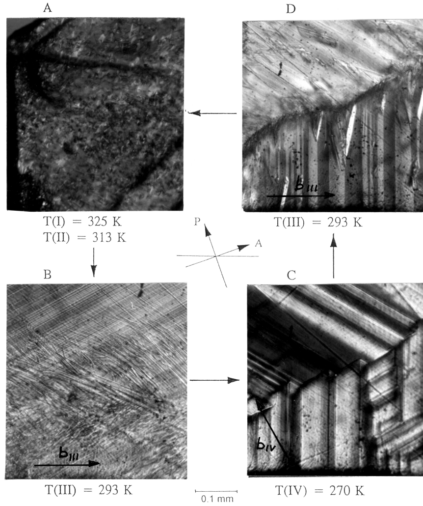
Figure 3. Thermal evolution of ferroelastic domains in (\text{NH}_4)_3\text{H}(\text{SeO}_4)_2 . The pictures present the sample surface in phases I, II-(A), III-(B), IV-(C) and again III (D). The arrows show the direction of temperature changes.
