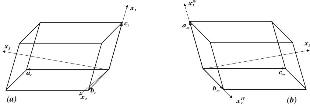
Figure 1. The unit cell of the (\text{NH}_4)_3\text{H}(\text{SeO}_4)_2 crystal in (a) triclinic phase III; (x_1, x_2, x_3) is the Cartesian coordinate system and (b) monoclinic phase IV with the Cartesian coordinate system (x_1^{IV}, x_2^{IV}, x_3) .
