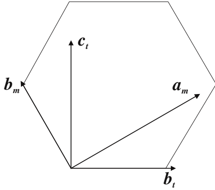
Figure 2. Projection of the lattice vectors in the triclinic phase III and the monoclinic phase IV on the (001) -plane in the hexagonal setting of phase II.
