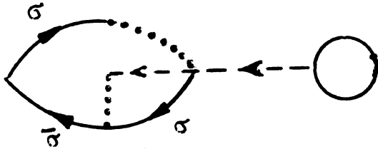
Figure 8. A second order correction to magnon Green function.
