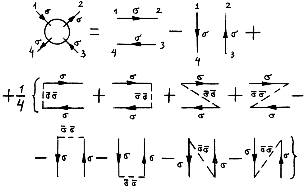
Figure 3. Graphic representation of \frac{1}{\mathcal{Z}} \frac{\delta^2 \mathcal{Z}}{\delta t_{12}^\sigma \delta t_{34}^\sigma} in zero approximation. Dashed lines denote plasmon Green functions (2.10).
