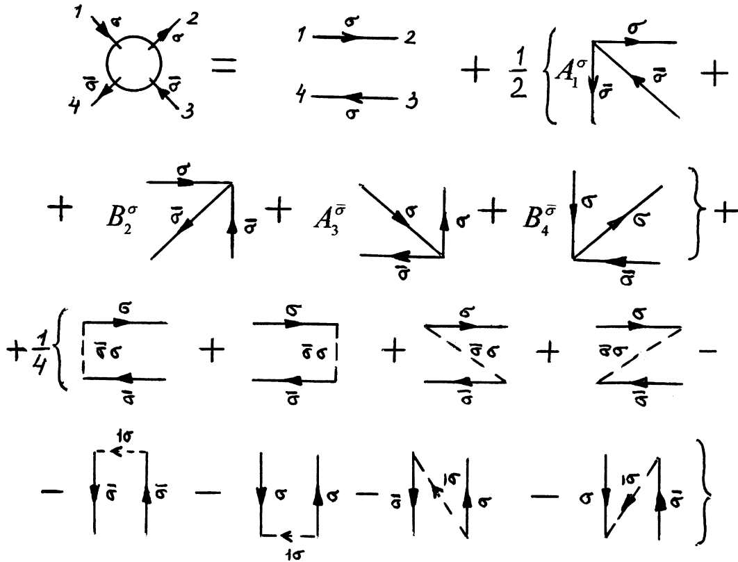
Figure 4. Graphic representation of \frac{1}{Z} \frac{\delta^2 Z}{\delta t_{12}^{\sigma} \delta t_{34}^{\bar{\sigma}}} in zero approximation. Dashed lines with an arrow denotes the magnon Green function (2.9).
