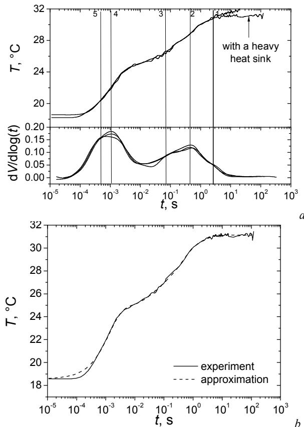
Fig. 6. Time dependence of dV/d\log(t) (a) and four-sectional approximation of LED no 1 temperature relaxation (b).
