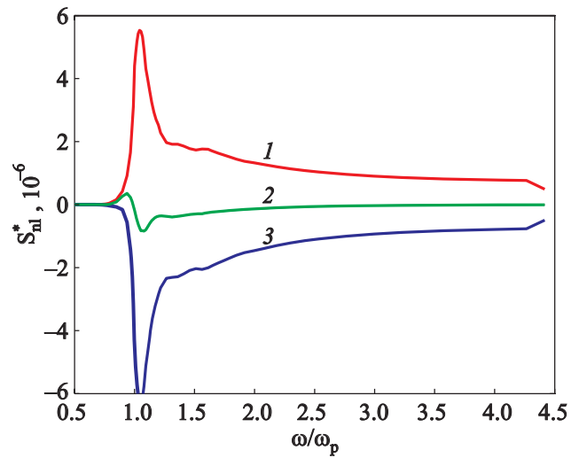
Fig. 4. Split of nonlinear interaction term S_{nl} (2) into F_k (1) and \Gamma_k N_k (3).
