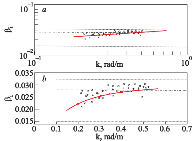
Fig. 2. Dimensionless wavenumber spectral coefficient \beta_i plotted in logarithmic scales (a) and linear scales (b), taken from [20]. Here crosses represent omnidirectional (averaged by angles) spectrum and dots correspond to \xi(k) = 2\beta_I u_* g^{-0.5} k^{-2.5} . The solid line on (a) and solid curve on (b) correspond to \xi(k) \simeq k^{-7/3} .
