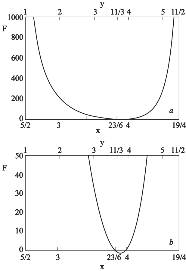
Fig. 1. Plot of function F(x) (a). Plot of function F(x) : zoom in the vertical direction (b).
