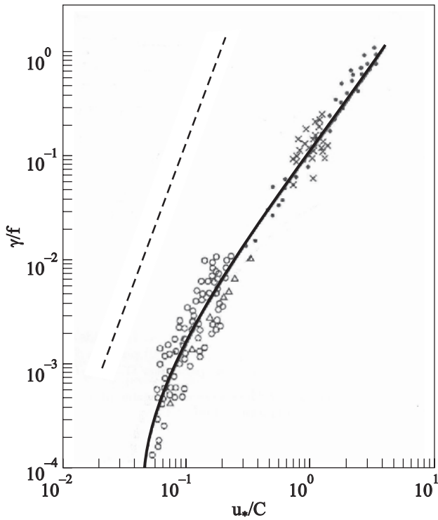
Fig. 3. Comparison of experimental data for the wind-induced growth rate 2\pi\gamma_{in}(\omega)/\omega taken from [26] and the damping due to four-wave interactions 2\pi\Gamma(\omega)/\omega , calculated for narrow in angle spectrum at \mu \simeq 0.05 using Eq. 6.11 (dashed line).
