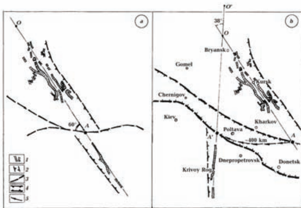
Model for formation of Pripyat-Dnieper-Donetsk system of formation of paleorifts: a — location of board's zones of paleorifts and structures of iron-ore formations in earlyproterozoics time (1000 m. years ago); b — present location (1 — magnetic anomalies in earlyproterozoics time (Krivoyrog's and Kursk series [Zankevich, 2006]; 2 — boundaries of proterozois geosynclines zone; 3 — proterozois fault in massif of the Sarmat's shield; 4 — boundaries fault of paleorifts; 5 — the trajectory of movement of conventional point A–A 1 ; O–O 1 — dislocation of rotation axis of the Ukrainian shield).
