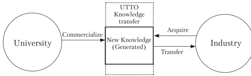
Fig. 1. Theoretical model
