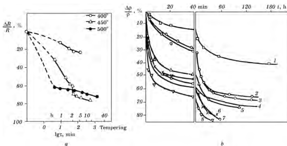
Fig. 12. The kinetics of the resistivity change of Cu-Ti alloys: a — with 4.45 wt.% Ti [9]; b — 4.7 wt.% Ti aged at temperatures: 1 — 340; 2 — 400; 3 — \epsilon = 50\% + 400 ; 4 — 500; 5 — 450; 6 — \epsilon = 12\% + 500 ; 7 — \epsilon = 50\% + 450 ; 8 — \epsilon = 50\% + 500 (°C) [48].
