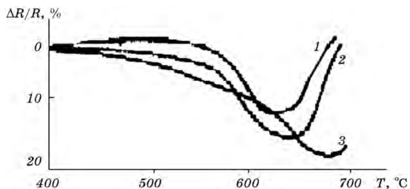
Fig. 23. The temperature dependence of the resistivity of the Cu-5.3 at.% Ti alloy under a pressure: 1 — 1.5; 2 — 2.54; 3 — 3.7 GPa [79].
