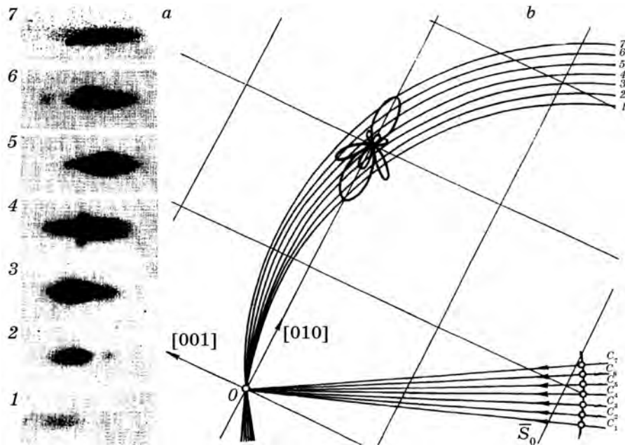
Fig. 8. a — the set of the diffuse scattering cross-sections near the 200 reflex of the Cu-5 at.% Ti alloy aged at 400°C, 8 h after rotating of the stationary single crystal on 18'. The Cu k_\alpha — radiation. Magnification \times 10 . b — the corresponding cross-sections of the diffuse scattering regions in the reciprocal space near the node 200 [39].
