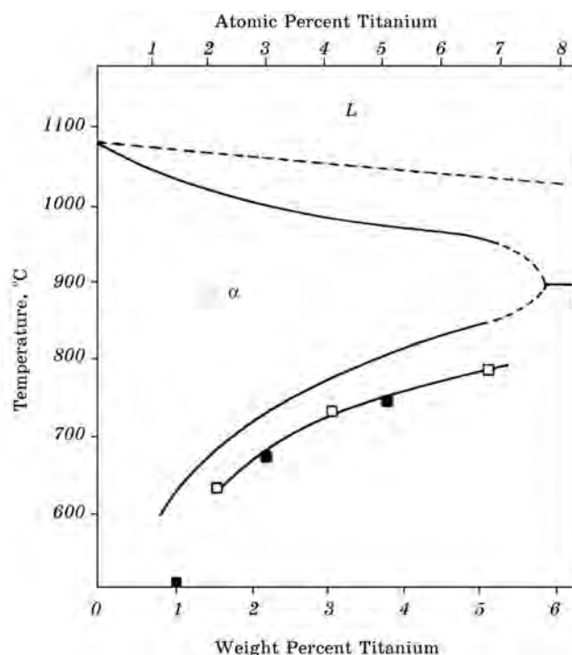
Fig. 3. The measured metastable \alpha' ( D1_n ) coherent solvus curve in Cu-rich region [25].
