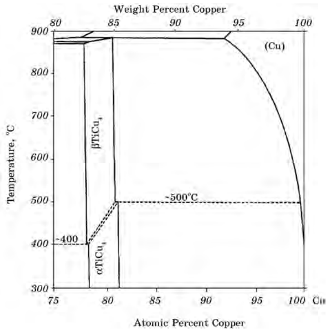
Fig. 2. The Cu-rich portion of Cu-Ti diagram showing the polymorphic transformation in Cu_4Ti phase [27].
