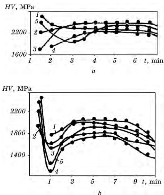
Fig. 29. The kinetics of the hardness reversion in Cu-5 at.% Ti alloy at T = 600^\circ\text{C} . (a) aged at the temperatures: 1 — 500^\circ\text{C} , 10 h; 2 — 550^\circ\text{C} , 30 min; 3 — 400^\circ\text{C} , 30 min; 4 — aging at 600^\circ\text{C} ; 5 — 400^\circ\text{C} , 10 h; the same at 700^\circ\text{C} (b) after aging at the temperatures: 1 — aging at 700^\circ\text{C} ; 2 — 400^\circ\text{C} , 30 min; 3 — 550^\circ\text{C} , 30 min; 4 — 500^\circ\text{C} , 10 h; 5 — 400^\circ\text{C} , 10 h [85].
