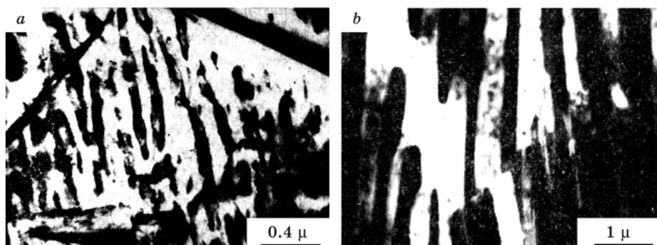
Fig. 11. The stable \beta -phase precipitation: a — in the Widmaschtett's form (indicated by arrows); b — as cell decomposition. The Cu-5.5 wt.% Ti alloy aged for 1 h at 600°C. Bright — field [29].
