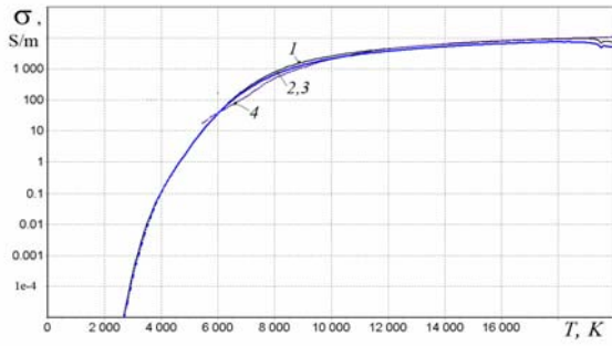
Fig. 1. Electrical conductivity of water plasma ( p = 1 bar). Curves 1-Lorentzian model (LM); 2- zero-density model (ZM); 3- dense model (DM); 4- data from [14]
