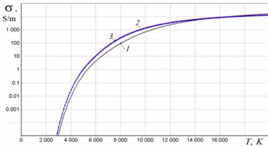
Fig. 2. Electrical conductivity of dense water plasma ( p = 200 bar). Curves: 1-LM; 2- ZM; 3-DM
