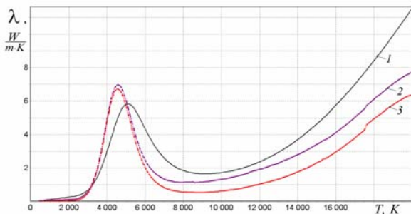
Fig. 4. Thermal conductivity of dense water plasma ( p = 200 bar). Curves 1-LM, 2- ZM, 3-DM
