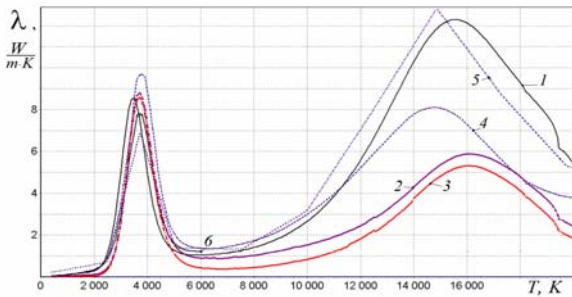
Fig. 3. Thermal conductivity of water plasma ( p = 1 bar). Curves: 1-LM; 2- ZM; 3-DM; 4- data from [14]; 5- [13]; 6-[15]
