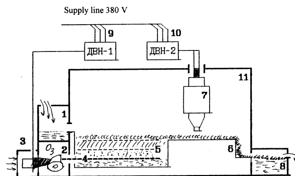
Fig. 1. The scheme of the disinfection device.
