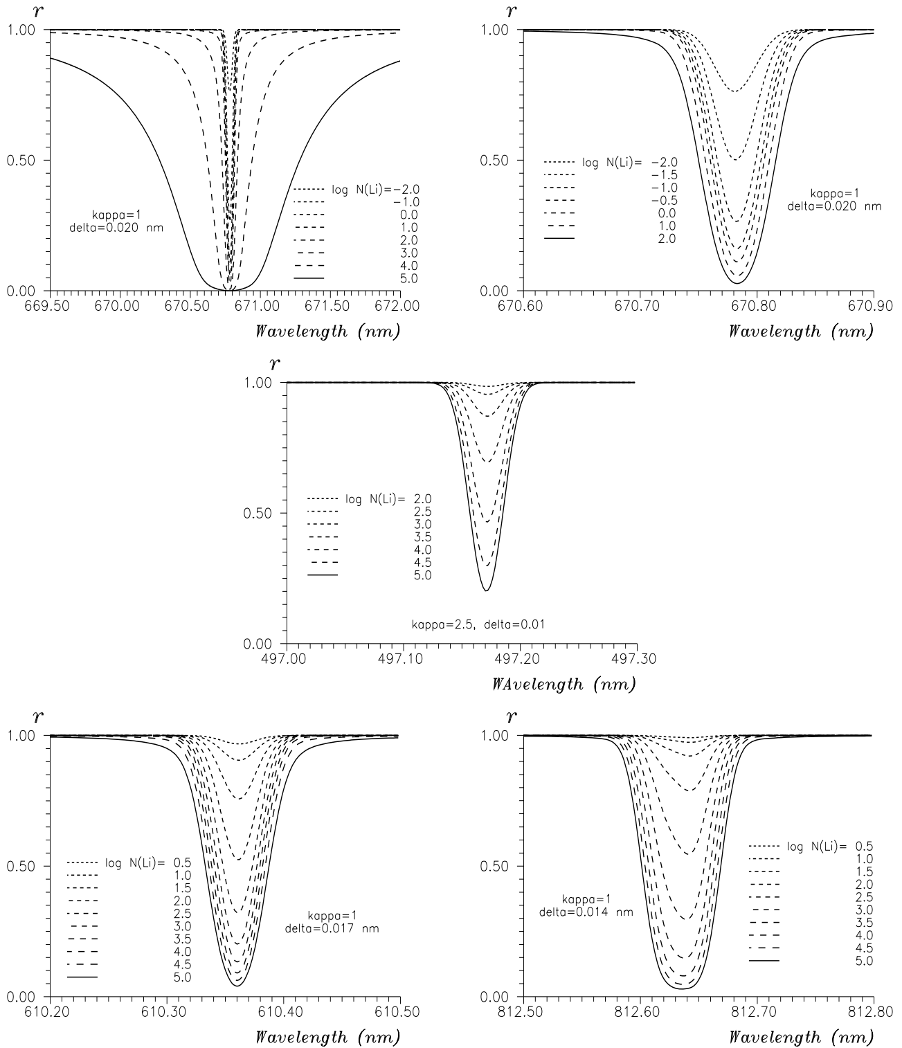
Figure 1. Profiles of LiI lines calculated with a model atmosphere 3000/0/0, C/O = 1.007 for various \log N(\text{Li})
