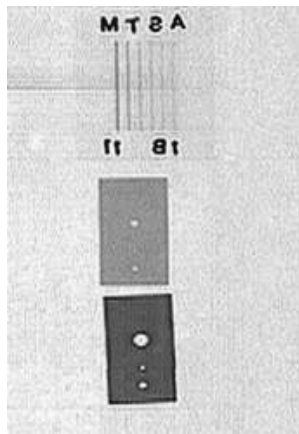
Fig.2. Wire and plate defectometers behind the 75 mm steel barrier
