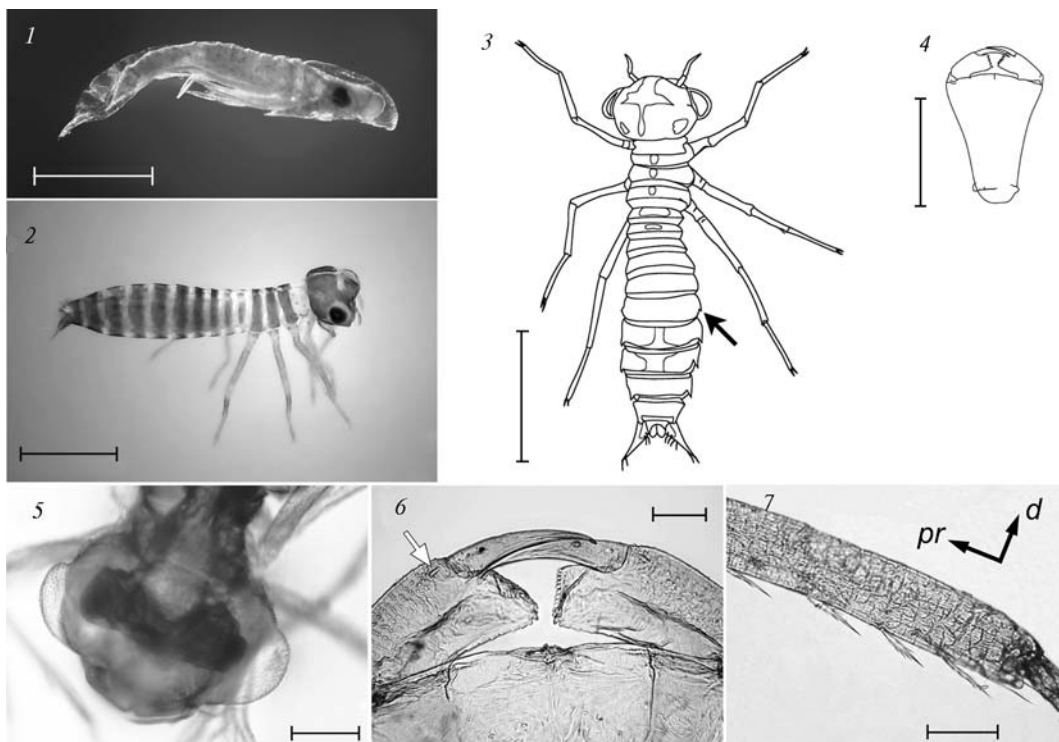
Fig. 2. Aeshnid instars reared from regular clutch: 1 – prolarva; 2–7 – first larva: 2, 3 – habitus, 4 – form of mask, 5 – head, 6 – labial palpi, 7 – first tarsus ( d – dorsal direction, pr – proximal direction). Black arrow indicates lateral thorn on S6, which is diagnostic character of some Aeshna species and Anaciaeschna isocetes . White arrow indicates short labial hair. Scale bars: 1, 2, 4 – 1.0 mm; 3, 6, 7 – 0.5 mm; 5 – 0.2 mm.
