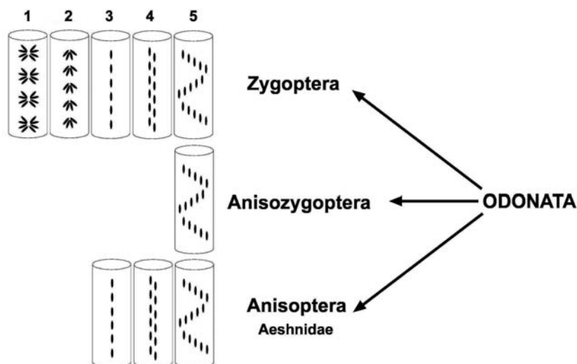
Fig. 3. Distribution of main patterns of regular endophytic clutches in recent odonate suborders: 1, 2 – complex linear, 3 – simple linear, 4 – simple zigzag, 5 – broad zigzag. According to Matushkina, Gorb (2000) for Zygoptera, Shimura (2005) for Anisozygoptera, and this study for Anisoptera.
