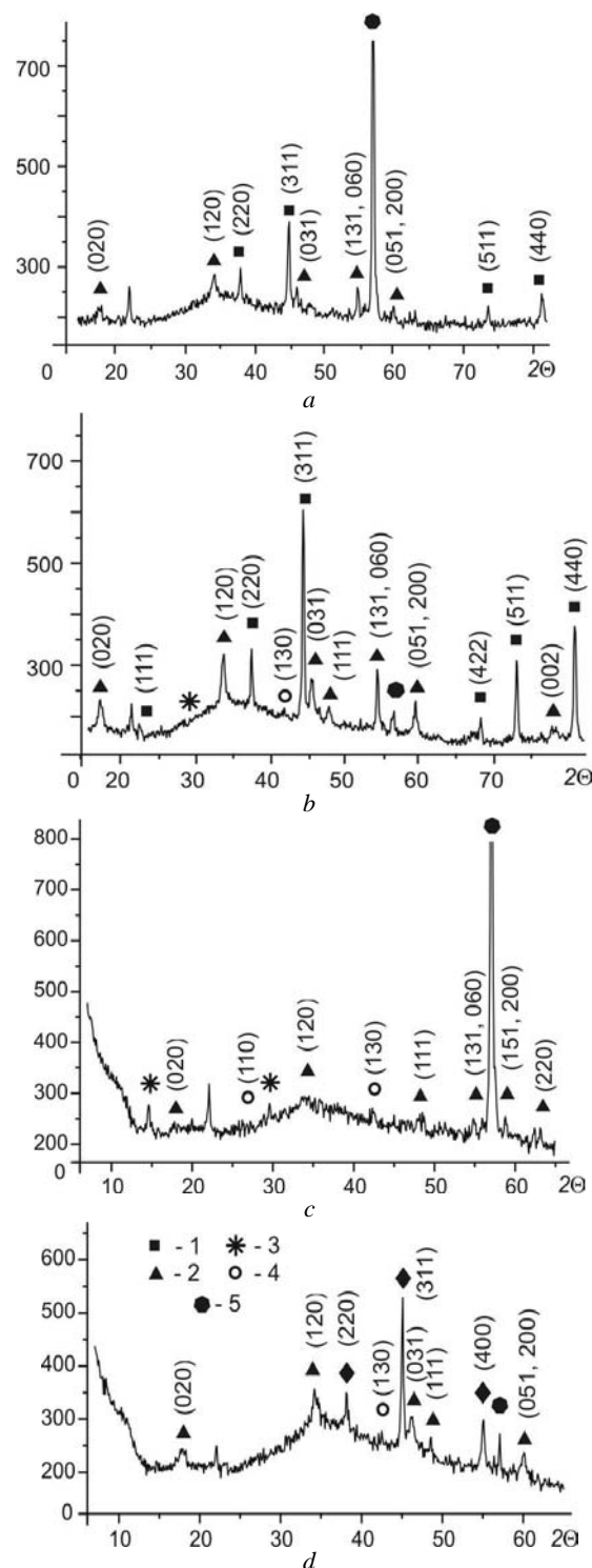
Fig. 4. XRD-data of surface structures formed on steel surface due to its contact with silver-containing dispersion medium: a – pH=6.5 after 5 h of contact of steel with solutions; b – pH=6.5 after 48 h; c – pH= 11.0 after 1 h; d – pH=11.0 after 70 h. Numbers correspond to the phases: 1 – magnetite FeFe 2 O 4 , 2 – lepidocrocite γ-FeOOH; 3 – Green Rust I; 4 – goethite α-FeOOH; 5 – iron Fe 0
