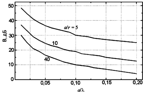
Fig. 2. HF radiation attenuation by metallic mesh
