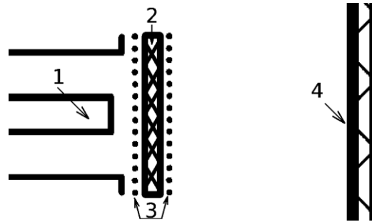
Fig. 10. Experiment 4 setup
