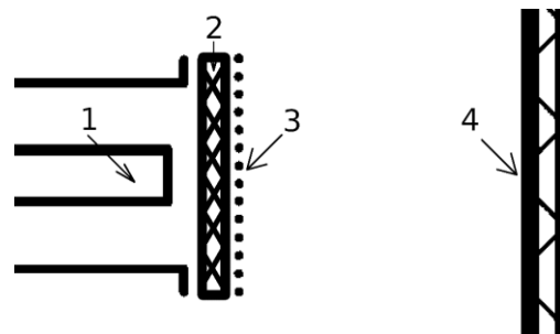
Fig. 5. Dielectric barrier in a vacuum diode
