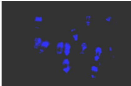
Fig. 8. Glass luminescence
