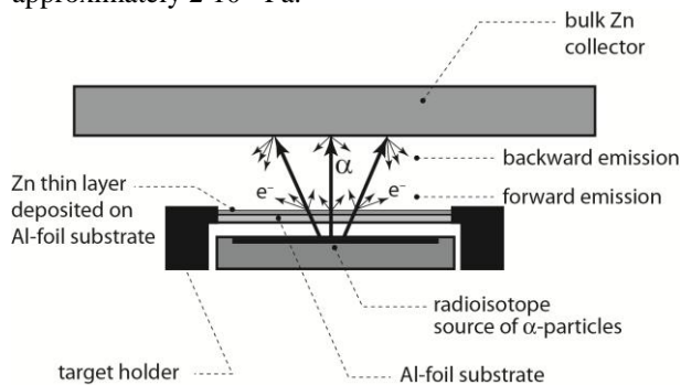
Fig. 1. Scheme of forward-backward electron emission experiments
