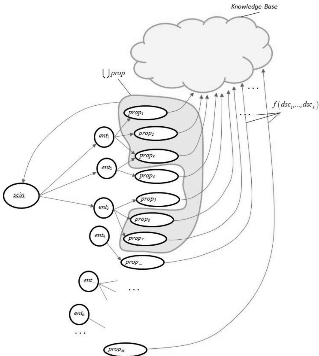
Figure 1. Formation of an element of an information scope ScIn in the form of aggregate properties as a function of descriptions Prop(Dsc) obtained from the knowledge base
