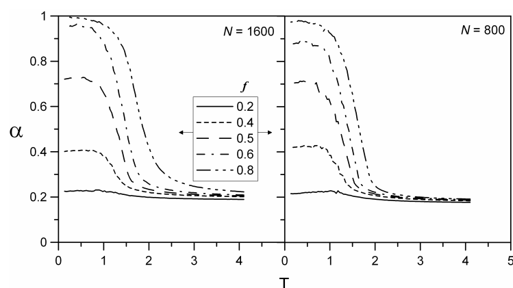
Figure 5. Relative gain in the number of vertically oriented molecules, \alpha , as a function of temperature, calculated for different amount fractions of the director molecules. The results of the figure correspond to enantiopure overlayers with a different number of adsorbed molecules indicated in each panel. These results are the averages over ten independent system replicas.
