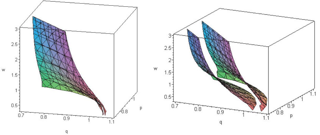
Figure 3. Left: The two “central” surfaces as implicit functions w = w(q,p) : one stems from equating \lambda_{p,q}^{(2)}(w) from Table 2 to the central value \lambda^{(2),\text{exp.}} = 0.57 in (14), the other stems from equating \lambda_{p,q}^{(3)}(w) from Table 3 to the central value \lambda^{(3),\text{exp.}} = 1.92 in (15). Notice mutual closeness of these “central” surfaces. Right: similar to the left panel, but now \lambda_{p,q}^{(2)}(w) is equated to \lambda_+^{(2),\text{exp.}} = 0.57 + 0.04 in (14) and \lambda_{p,q}^{(3)}(w) to \lambda_-^{(3),\text{exp.}} = 1.92 - 0.49 in (15).
