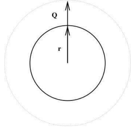
Figure 4. If the electric force is harmonic, then, for critical the magnetic field, all trajectories are circular, and are determined by the motion of the guiding center.
