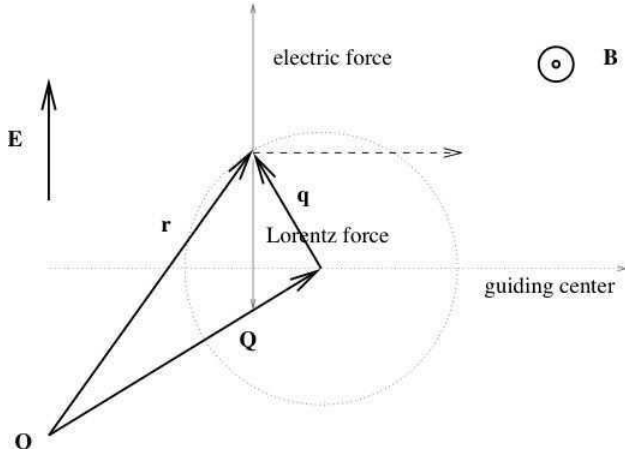
Figure 3. In a constant electromagnetic field, the electric and the Lorentz forces cancel in the critical case. The motion around the guiding center is “frozen” and the particle moves according to the Hall law.
