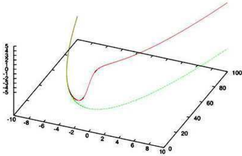
Figure 5. The anomalous velocity term deviates the trajectory from the plane. Most contribution to the shift comes when the momentum is small, i.e., when the particle passes close to the “ p -monopole”.
