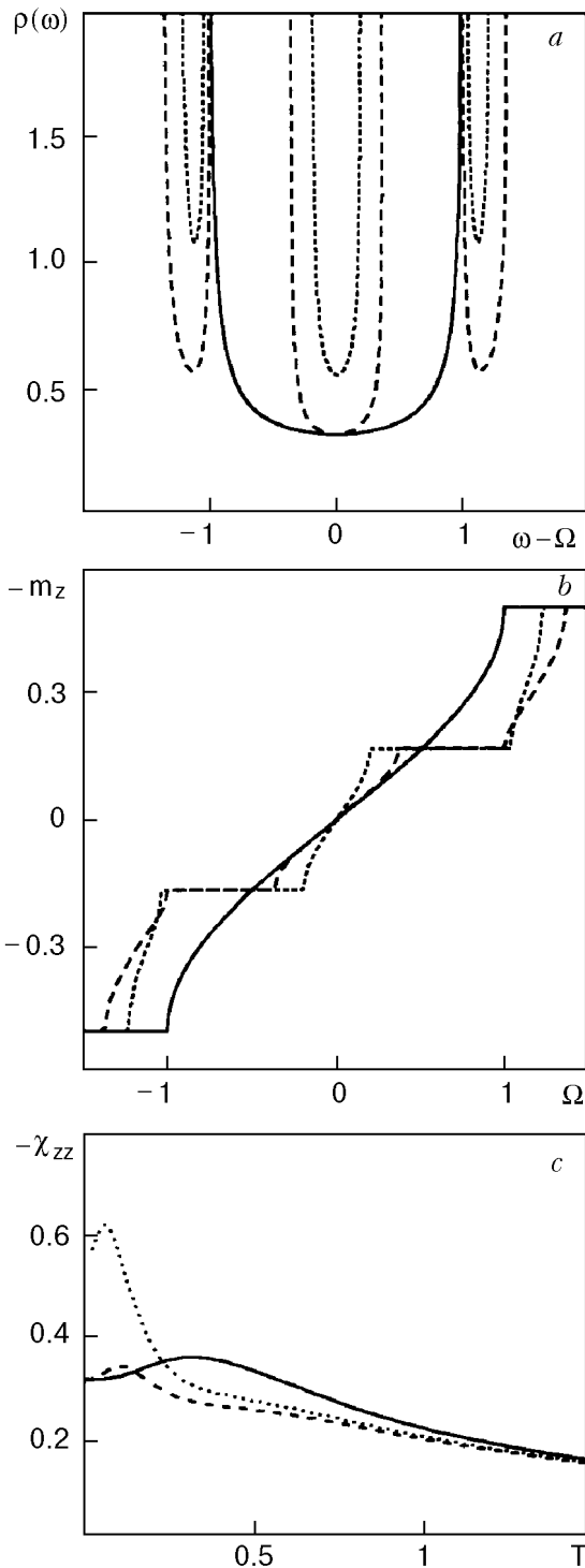
Fig. 1. Density of states (a), transverse magnetization versus transverse field \Omega at T = 0 (b), and static transverse linear susceptibility versus temperature at \Omega = 0 (c), for the nonuniform chain \Omega_1 \Omega_2 \Omega_3 \Omega_1 \Omega_2 \Omega_3 \dots , I_1 = 0.5 , I_2 = 0.5 , I_3 = 0.5 (solid lines); I_2 = 0.5 , I_3 = 1 (dashed lines); I_2 = 0.25 , I_3 = 1 (dotted lines).
