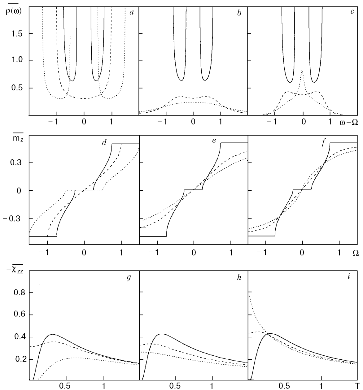
Fig. 3. Density of states ( a, b, c ), transverse magnetization versus transverse field \Omega at T = 0 ( d, e, f ), and static transverse linear susceptibility versus temperature at \Omega = 0 ( g, h, i ), for the nonuniform random chain \Omega_{01}\Gamma_1 I_1 \Omega_{02}\Gamma_2 I_2 \Omega_{01}\Gamma_1 I_1 \Omega_{02}\Gamma_2 I_2 \dots , I_1 = 0.5 , \Omega_{01} = \Omega_{02} = \Omega . a, d, g : non-random case \Gamma_1 = \Gamma_2 = 0 , I_2 = 0.25 (solid lines), I_2 = 0.5 (dashed lines), I_2 = 1 (dotted lines); b, e, h : uniform disorder I_2 = 0.25 , \Gamma_1 = \Gamma_2 = 0 (solid lines), \Gamma_1 = \Gamma_2 = 0.5 (dashed lines), \Gamma_1 = \Gamma_2 = 1 (dotted lines); c, f, i : nonuniform disorder I_2 = 0.25 , \Gamma_1 = 0 , \Gamma_2 = 0 (solid lines), \Gamma_2 = 0.5 (dashed lines), \Gamma_2 = 1 (dotted lines).
