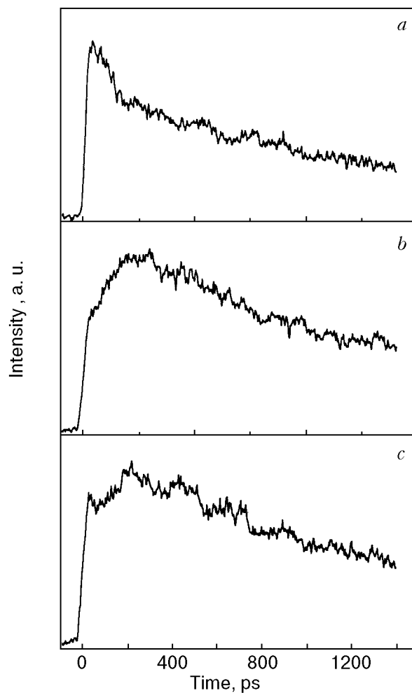
Fig. 5. Time-resolved fluorescence decay of the fluorescence bands of C_{60} in Ar matrices belonging to the different emitting characters: h_u(4) of the G_g character (a); t_{1u}(4) of the T_{1g} character (b), and h_u(1) of the T_{2g} character (c).
