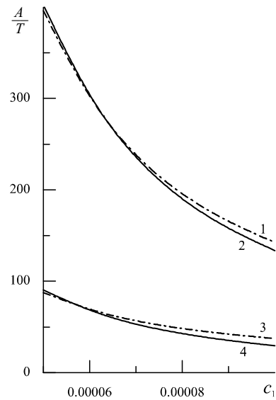
Figure 2. The dependence of the vapor-to-liquid nucleation barrier on the concentration of excited atoms c_1 at two temperatures T = 0.6T_c(0) (curves 1 and 2) and T = 0.8T_c(0) (curves 3 and 4). The curves 1 and 3 were obtained using equation (1), the curves 2 and 4 were obtained using equation (2).
